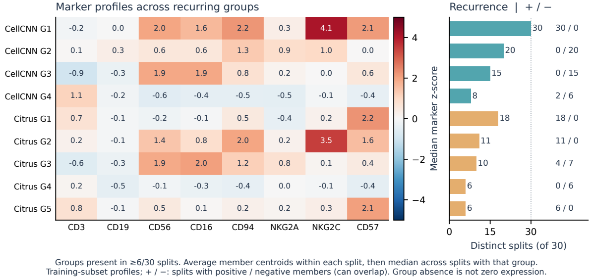
Figure S7: All retained CellCNN and Citrus centroid groups, with their marker summaries and recurrence. These are retrospective training-subset groups, not the held-out cell profiles of the main report.
