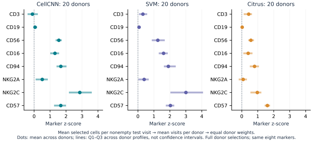
Figure S8: Held-out selected-cell profiles: dots are means across equally weighted donors, and lines are Q1-Q3 of donor profiles, not confidence intervals. The contribution count is 20 donors for each method.
