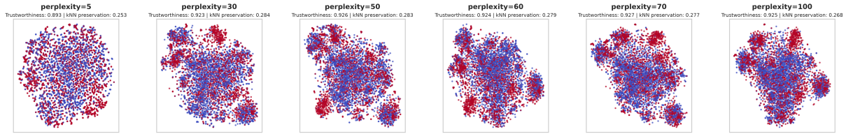
Figure S3: t-SNE on the 5,000-cell sweep subset. Left to right: perplexities 5, 30, 50, 60, 70 and 100; numerical quality measures are in Table S4. Red: CMV-positive donors; blue: negative donors. Perplexity changes the neighbourhood scale and visual organisation. The layouts are not independently annotated populations.
