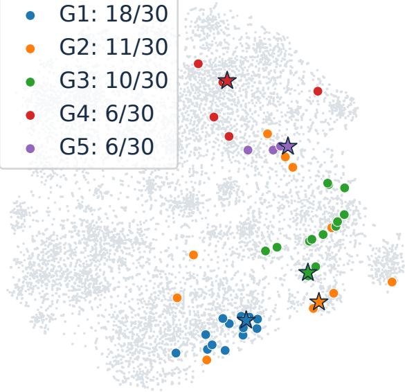
Citrus
