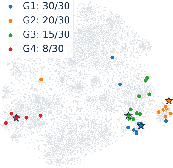
CellCNN
