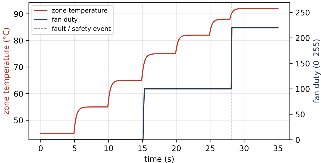
Heat-soak ramp: zone temperature and fan response
