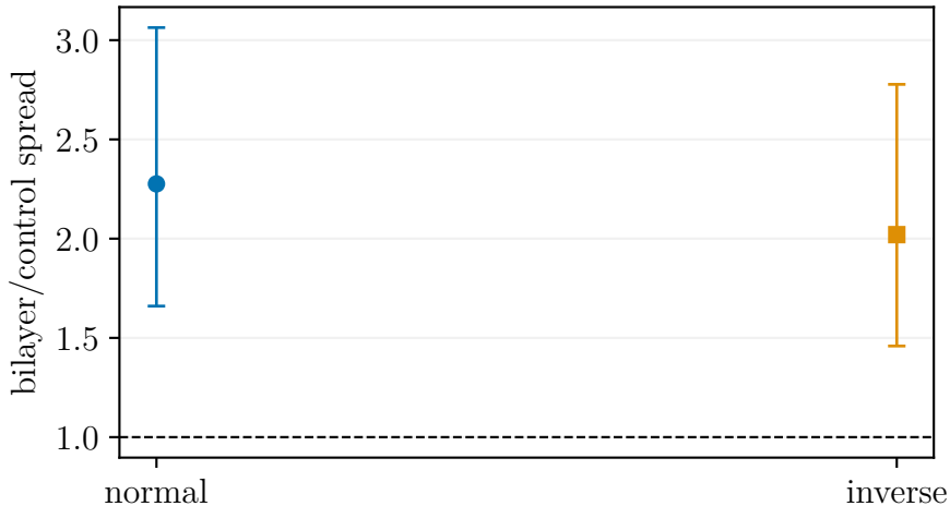
Replica-bootstrap test of single-scale collapse
