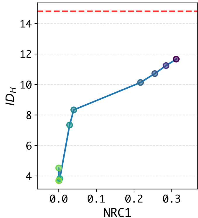
Humanoid_walk-50K ( n = 21 )
