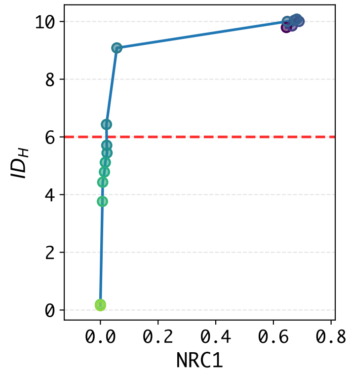
Cheetah_run-20K ( n = 6 )
