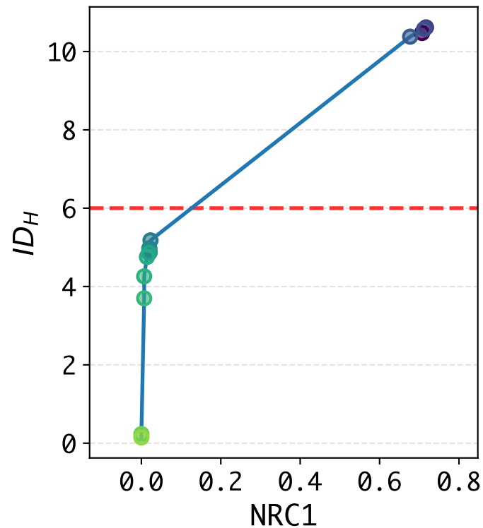
Cheetah_run-80K ( n = 6 )
