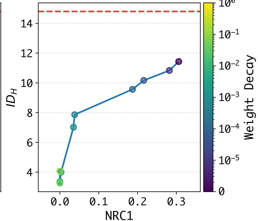
Humanoid_walk-100K ( n = 21 )
