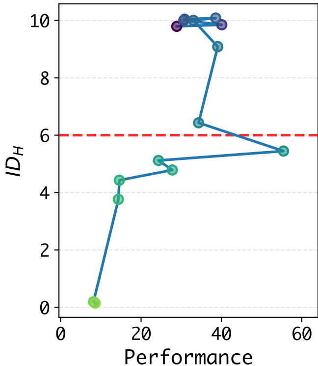
Cheetah_run-20K ( n = 6 )
