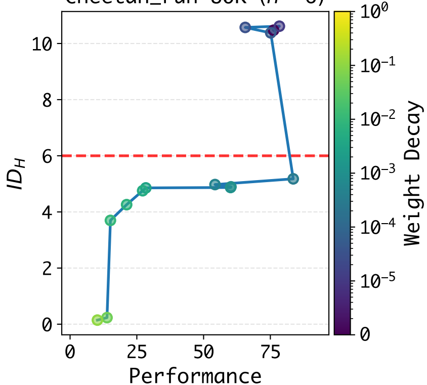
Cheetah_run-80K ( n = 6 )
