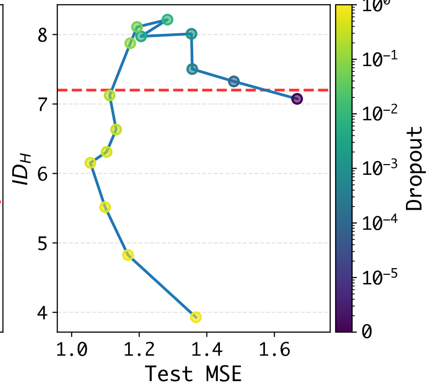
Ant-1K ( n = 8 )
