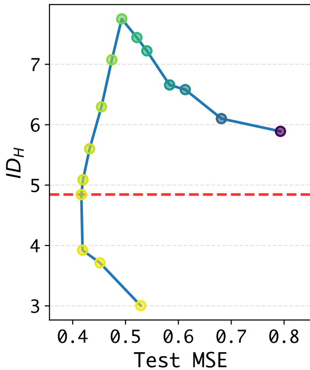
Halfcheetah-1K ( n = 6 )
