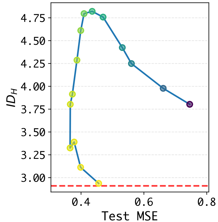
Hopper-1K ( n = 3 )
