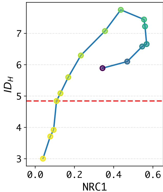
Halfcheetah-1K ( n = 6 )
