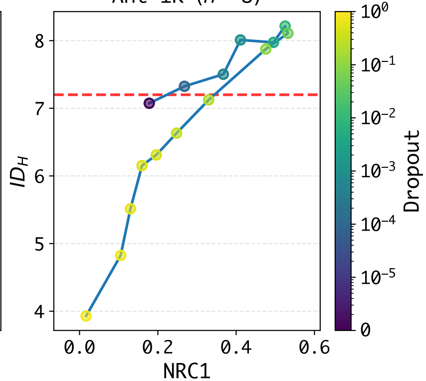
Ant-1K ( n = 8 )
