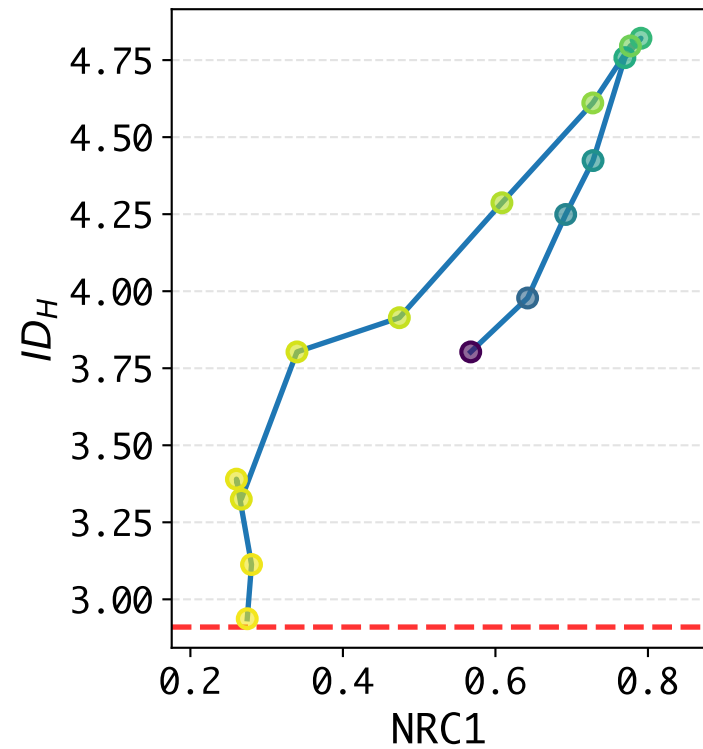
Hopper-1K ( n = 3 )
