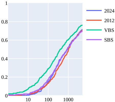
Fraction Instances Solved
