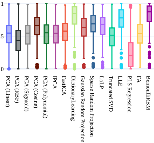
Mean Rank
