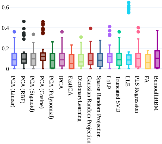
V-Measure
