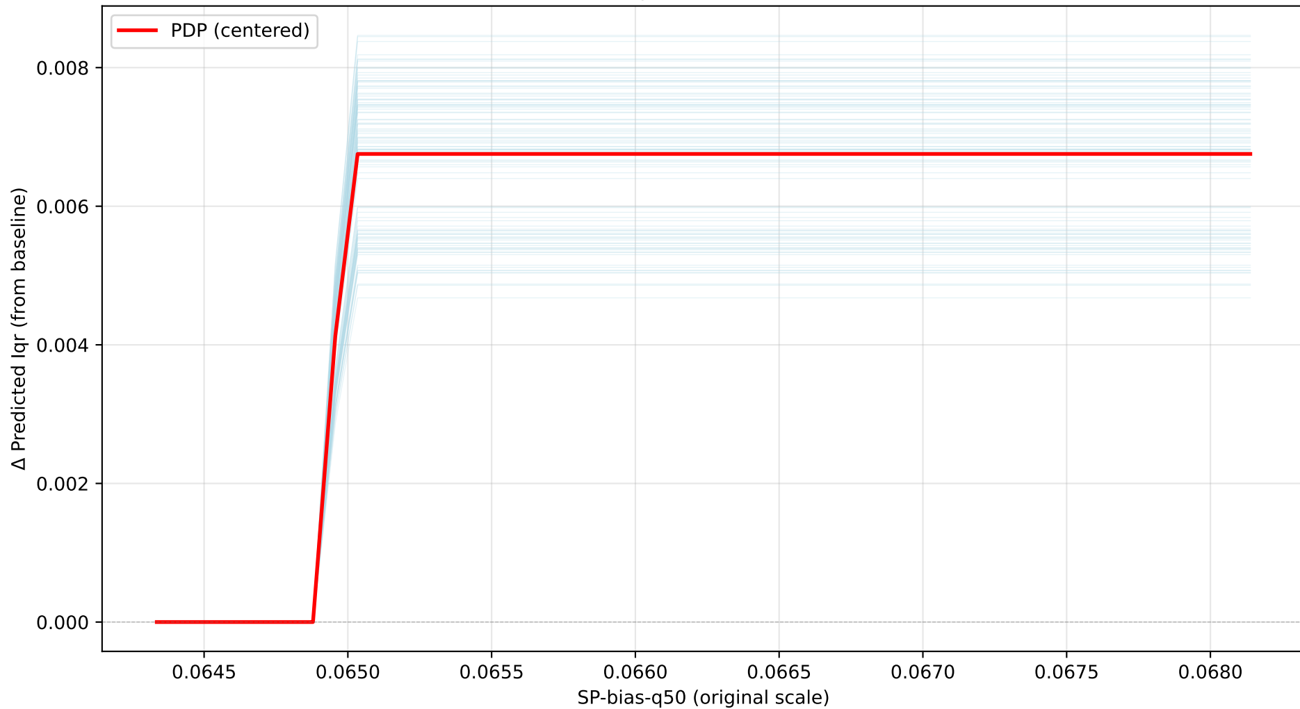
Centered ICE Curves for SP-bias-q50 (lqr) \Delta range: 0.008648 | Feature range: [0.064, 0.068]
