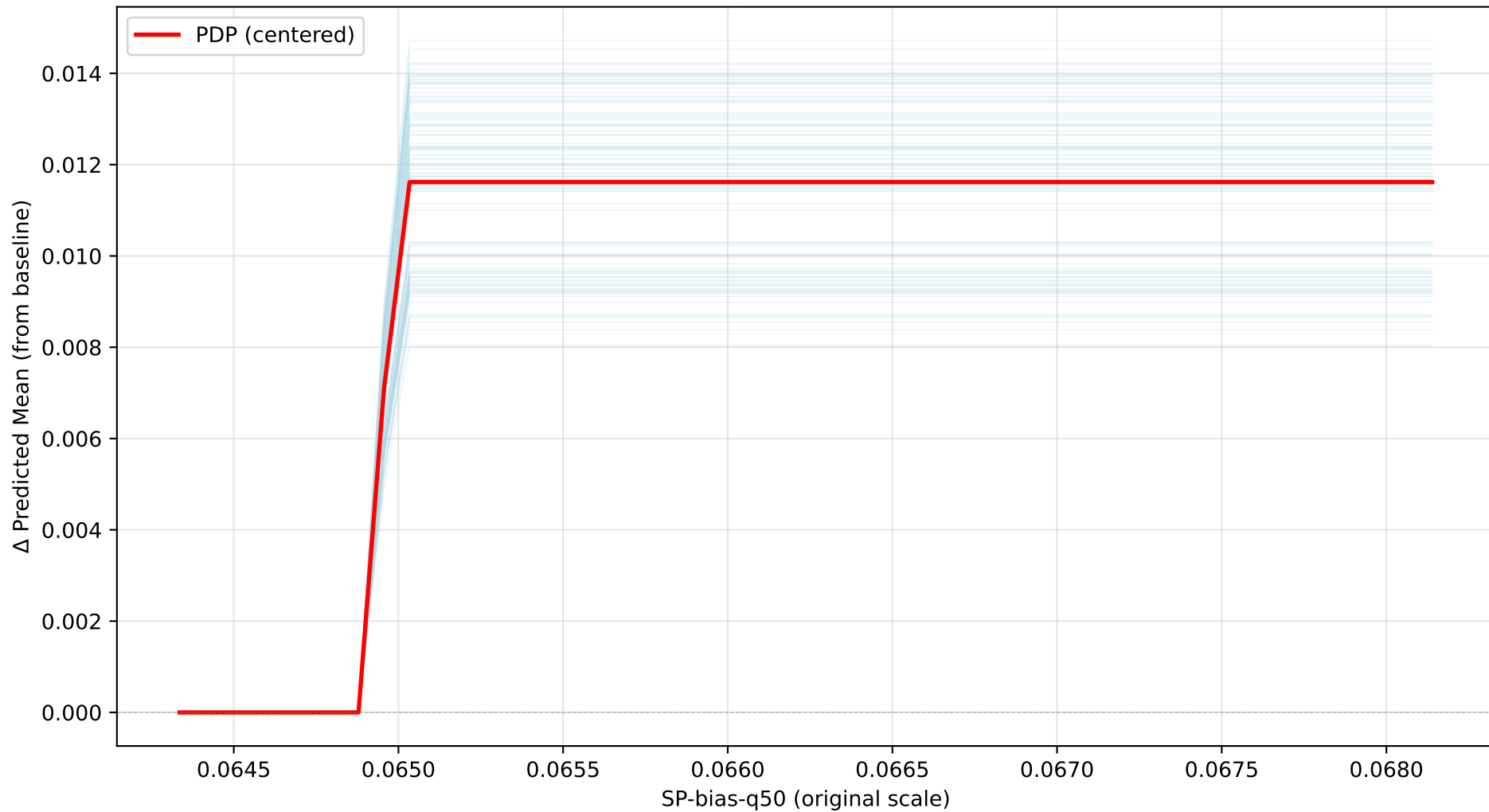
Centered ICE Curves for SP-bias-q50 (Mean) \Delta range: 0.014874 | Feature range: [0.064, 0.068]
