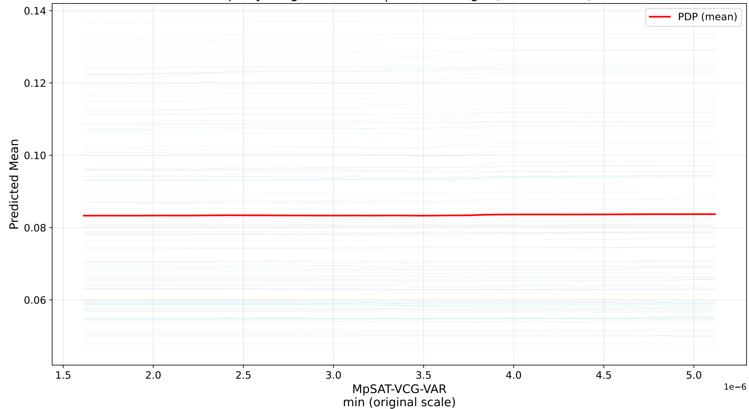
ICE Curves for MpSAT-VCG-VAR-min (Mean) Property range: 0.103640 | Feature range: [0.000, 0.000]
