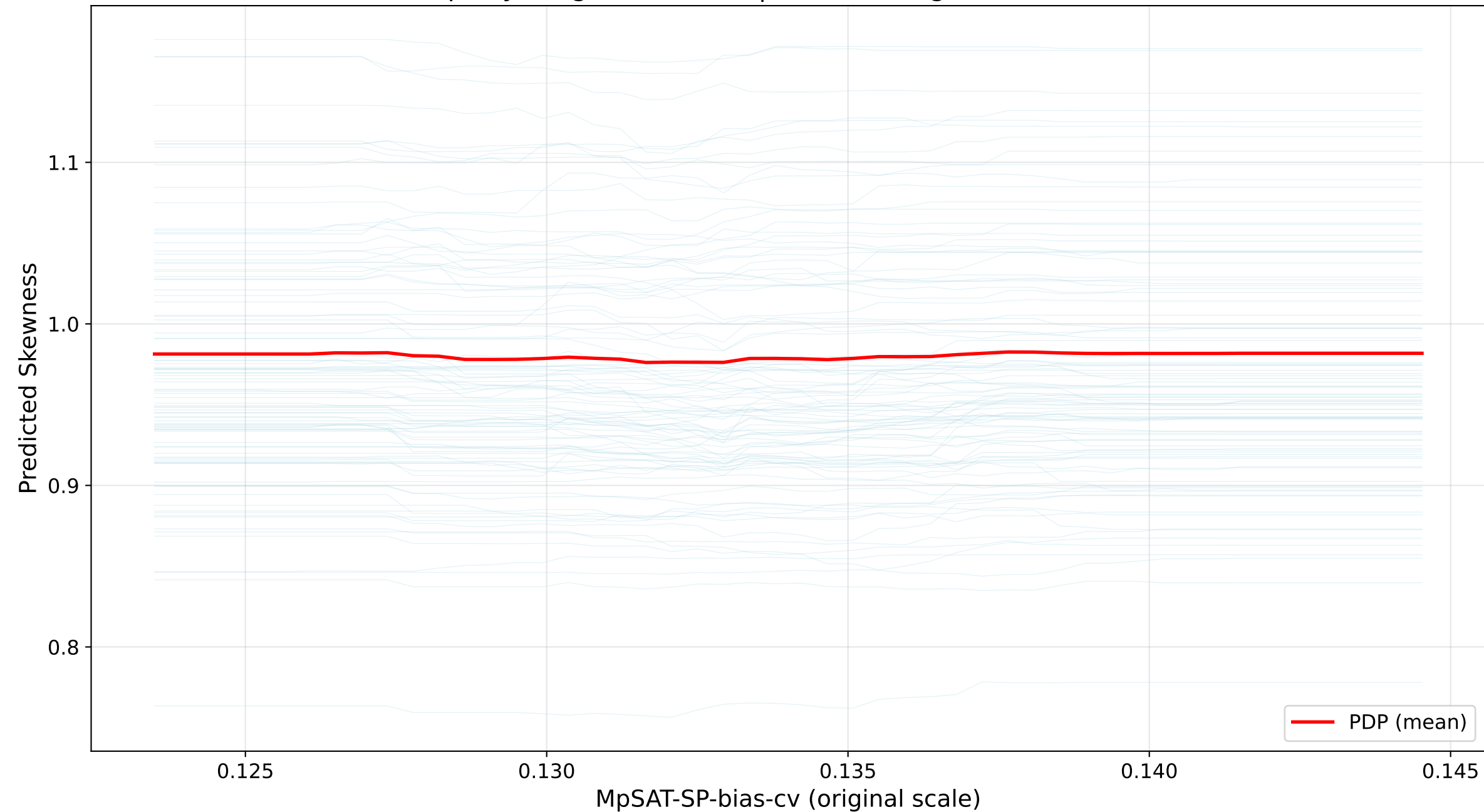
ICE Curves for MpSAT-SP-bias-cv (Skewness) Property range: 0.426331 | Feature range: [0.123, 0.145]
