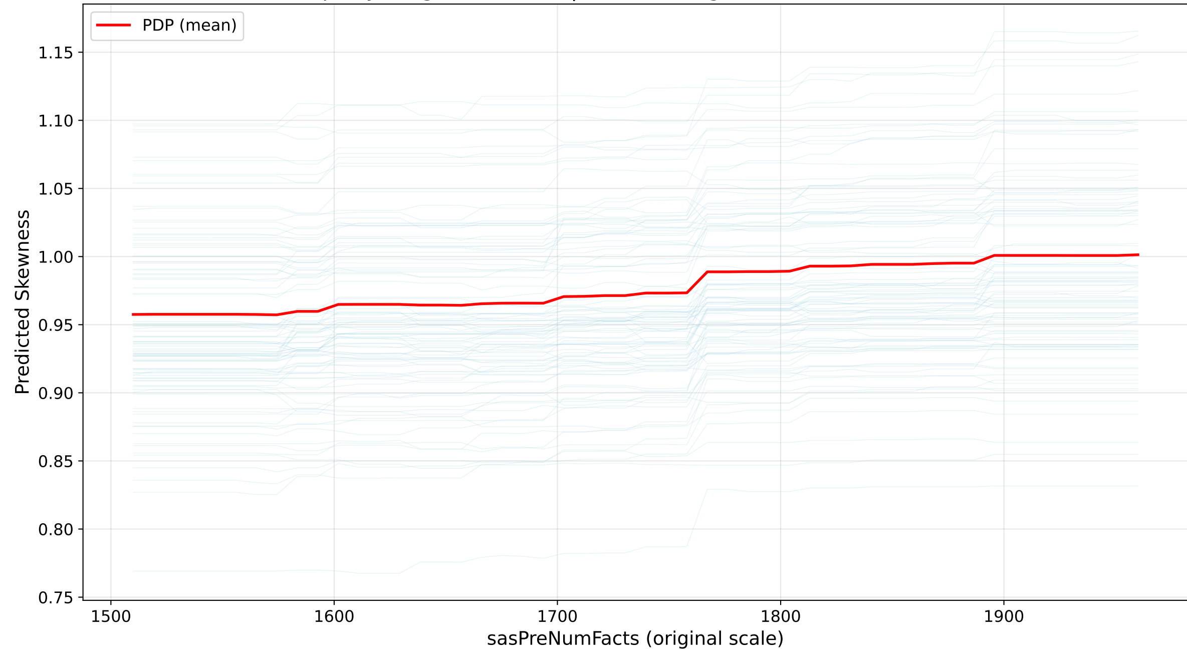
ICE Curves for sasPreNumFacts (Skewness) Property range: 0.450152 | Feature range: [1510.000, 1960.000]
