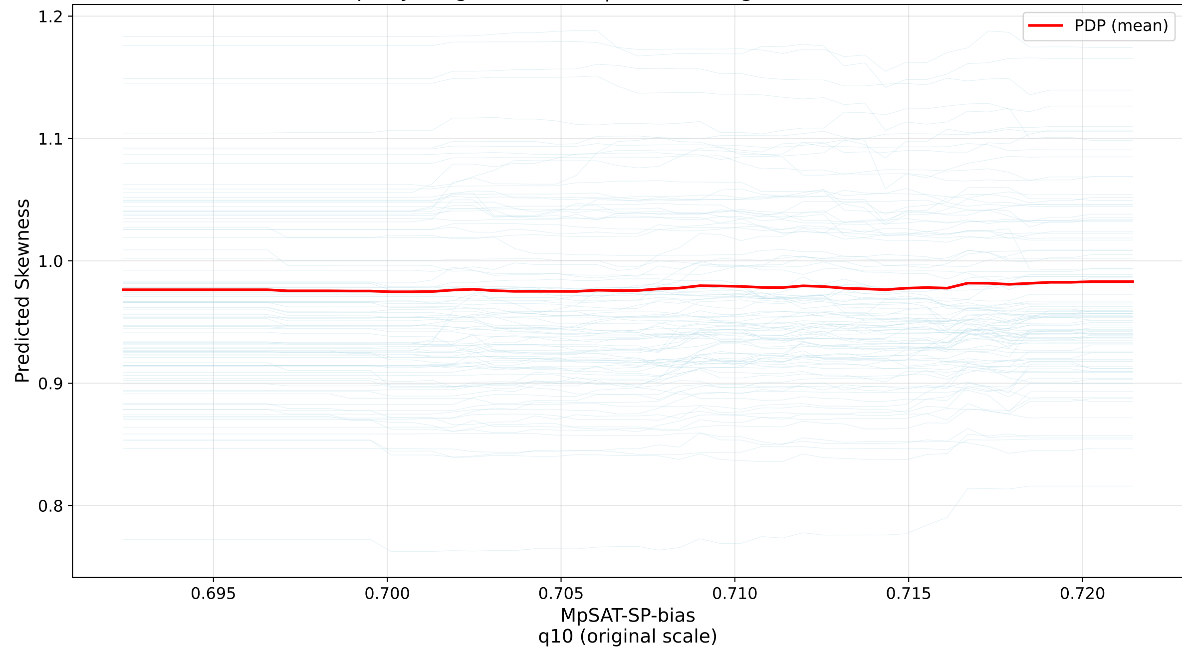
ICE Curves for MpSAT-SP-bias-q10 (Skewness) Property range: 0.439642 | Feature range: [0.692, 0.721]
