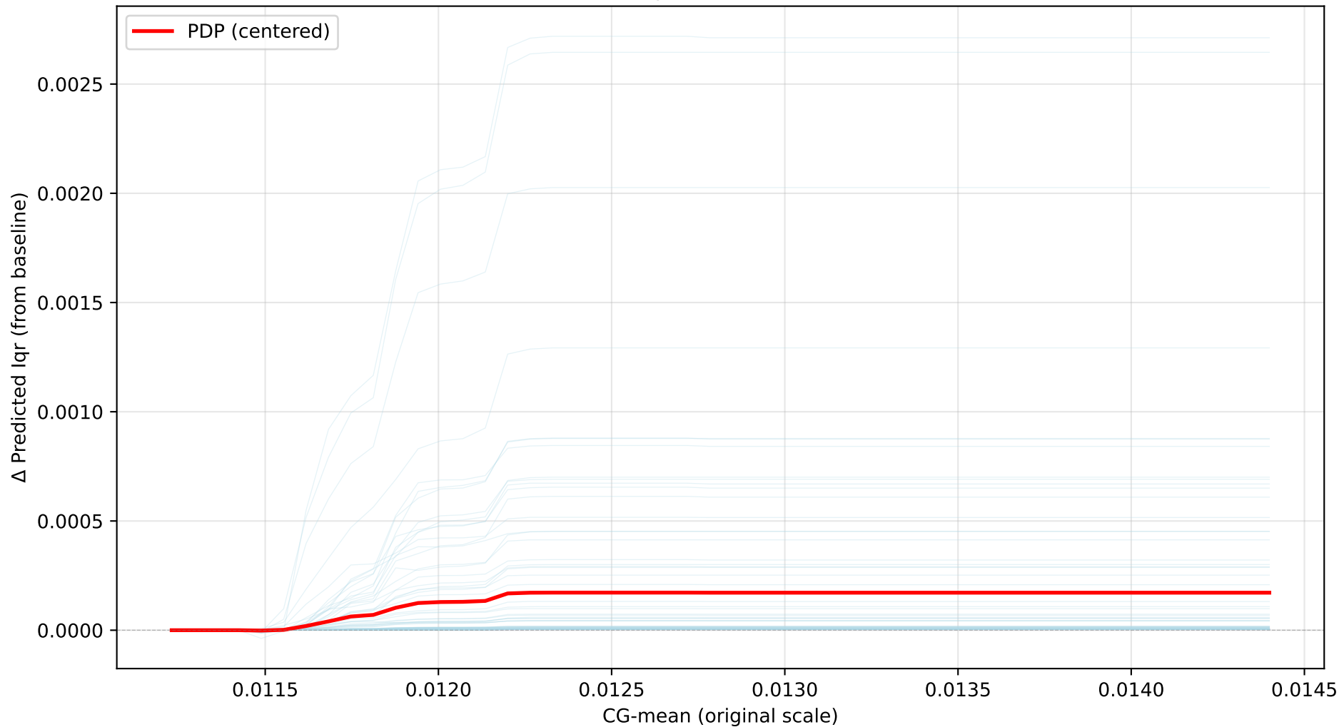
Centered ICE Curves for CG-mean (lqr) \Delta range: 0.003450 | Feature range: [0.011, 0.014]
