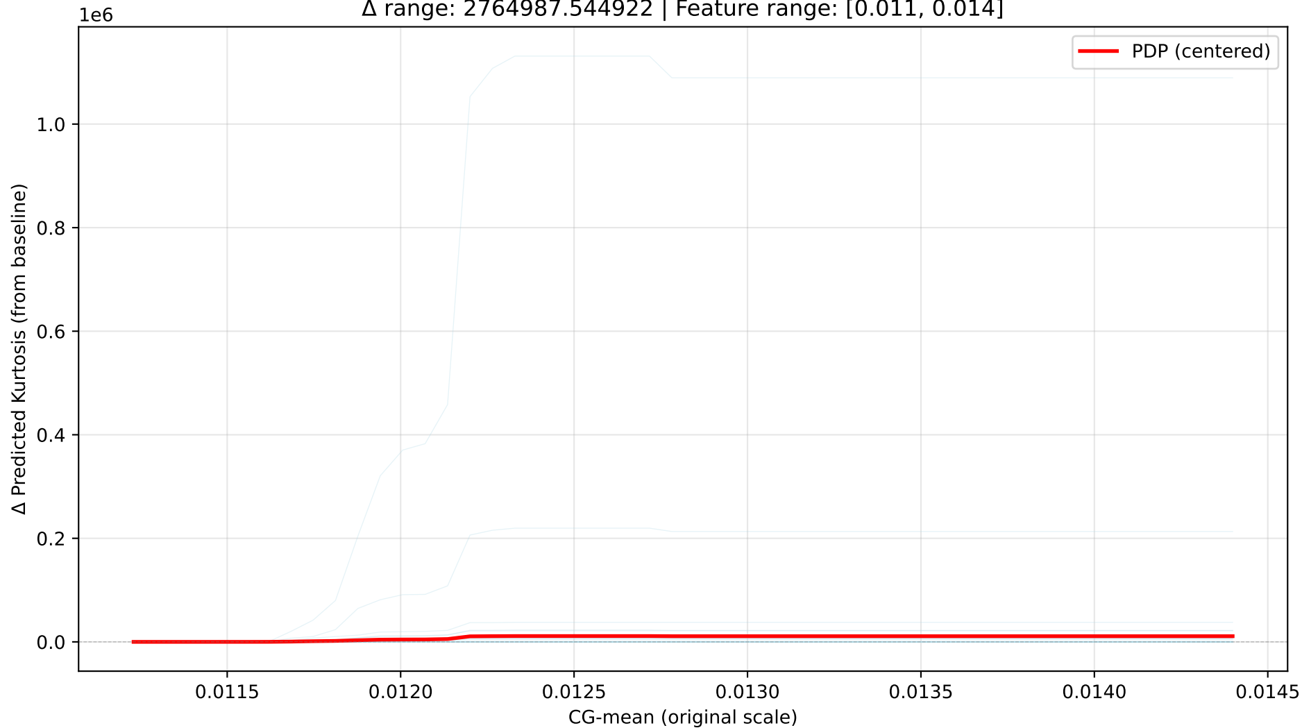
Centered ICE Curves for CG-mean (Kurtosis) \Delta range: 2764987.544922 | Feature range: [0.011, 0.014]
