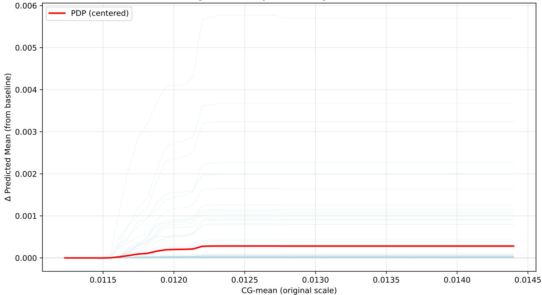
Centered ICE Curves for CG-mean (Mean) \Delta range: 0.005920 | Feature range: [0.011, 0.014]
