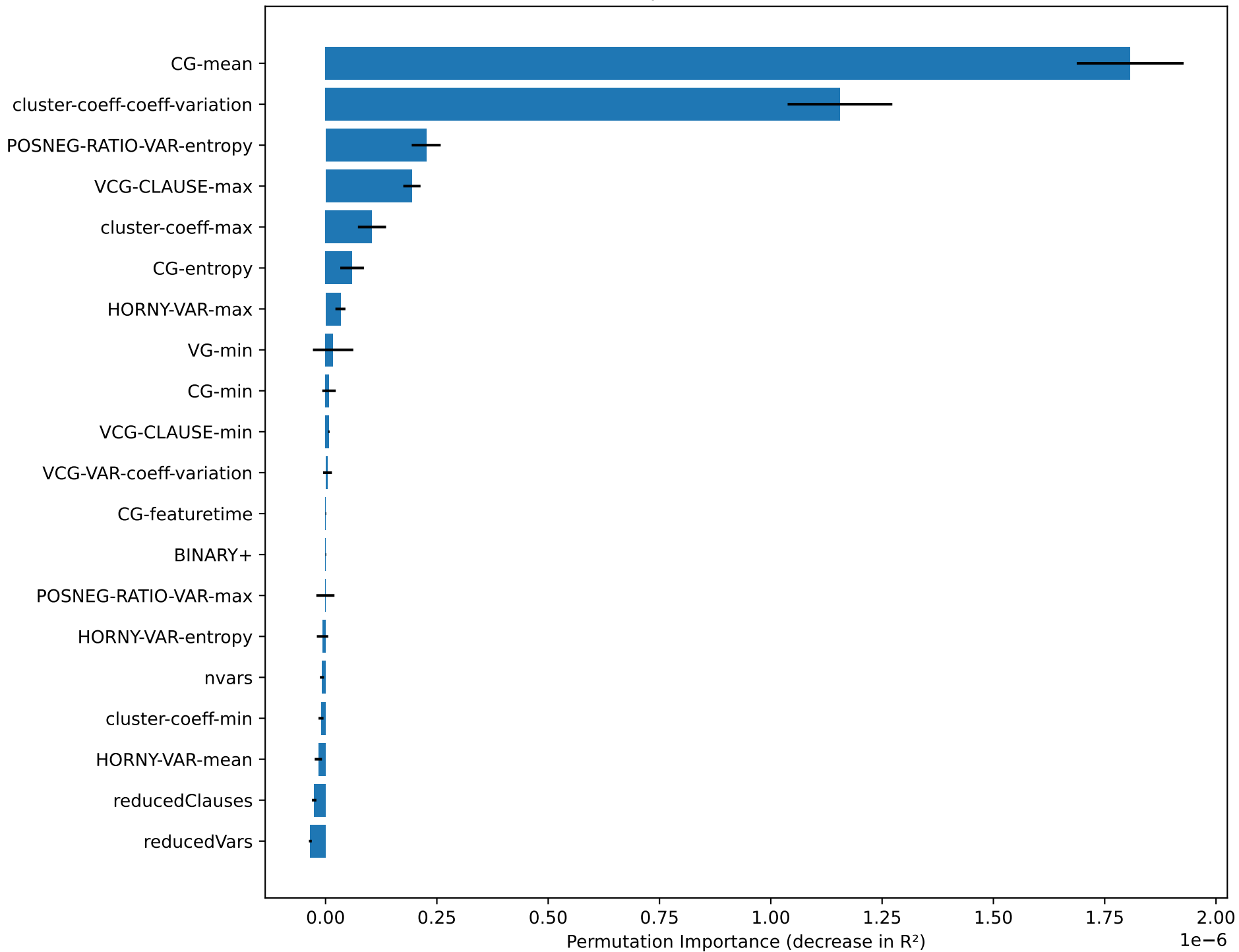
Feature Importance for Mean Prediction
