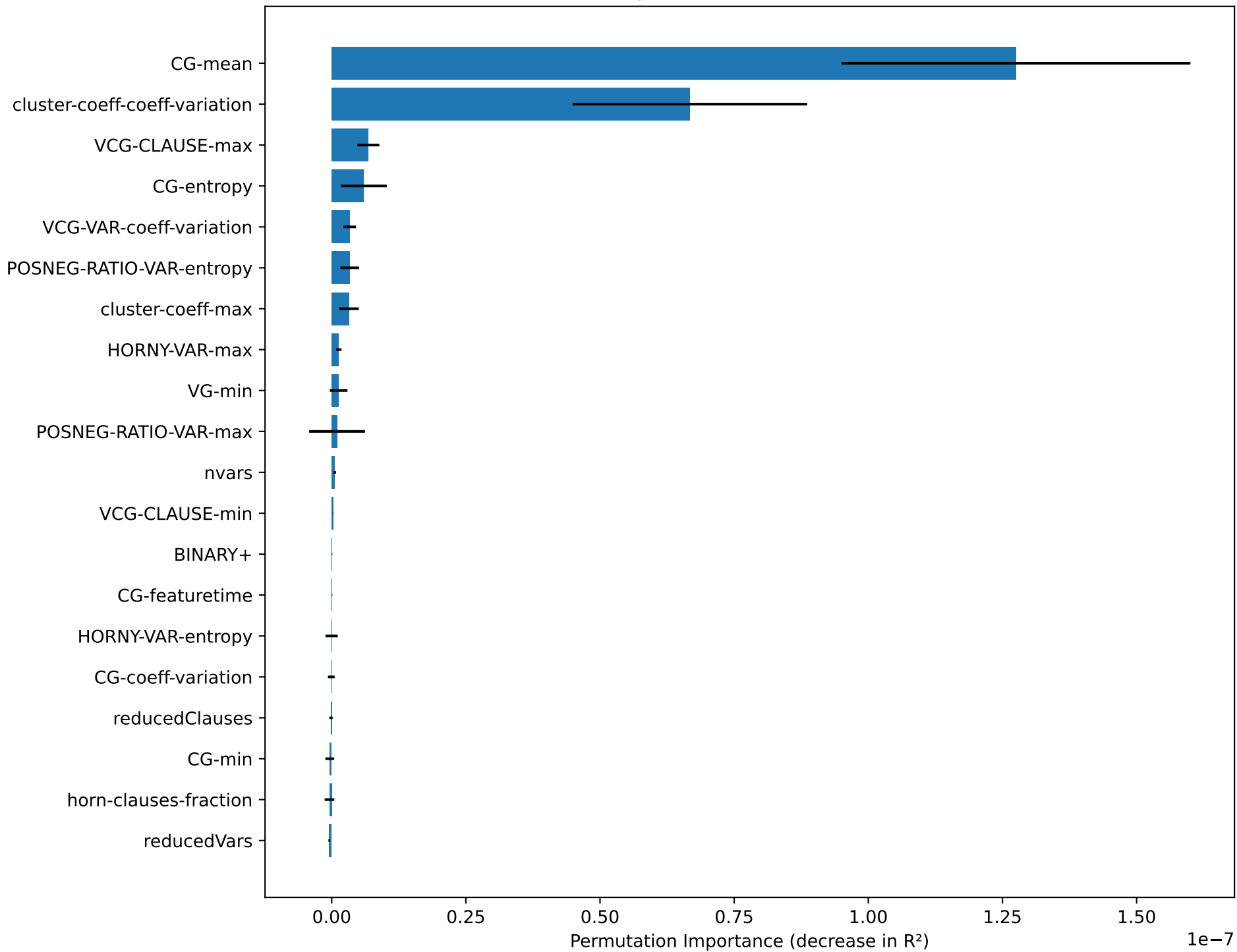
Feature Importance for Variance Prediction
