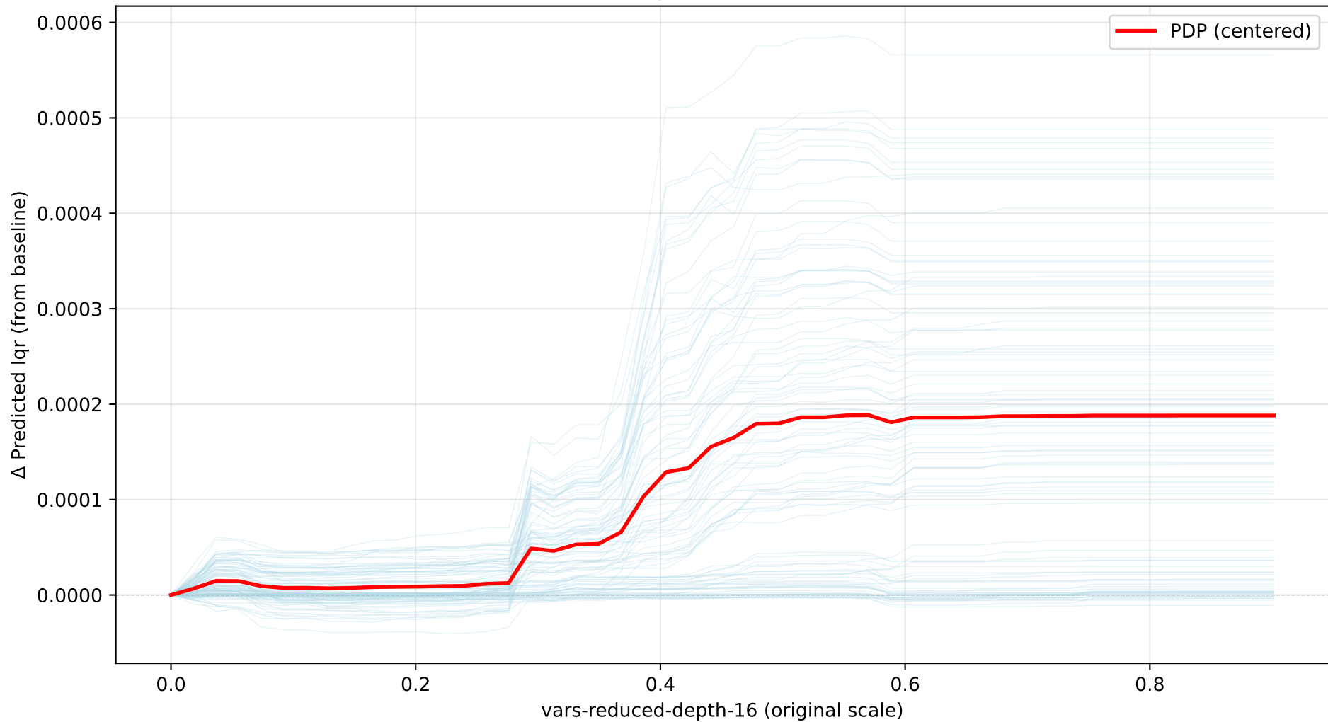
Centered ICE Curves for vars-reduced-depth-16 (lqr) \Delta range: 0.000801 | Feature range: [0.000, 0.901]
