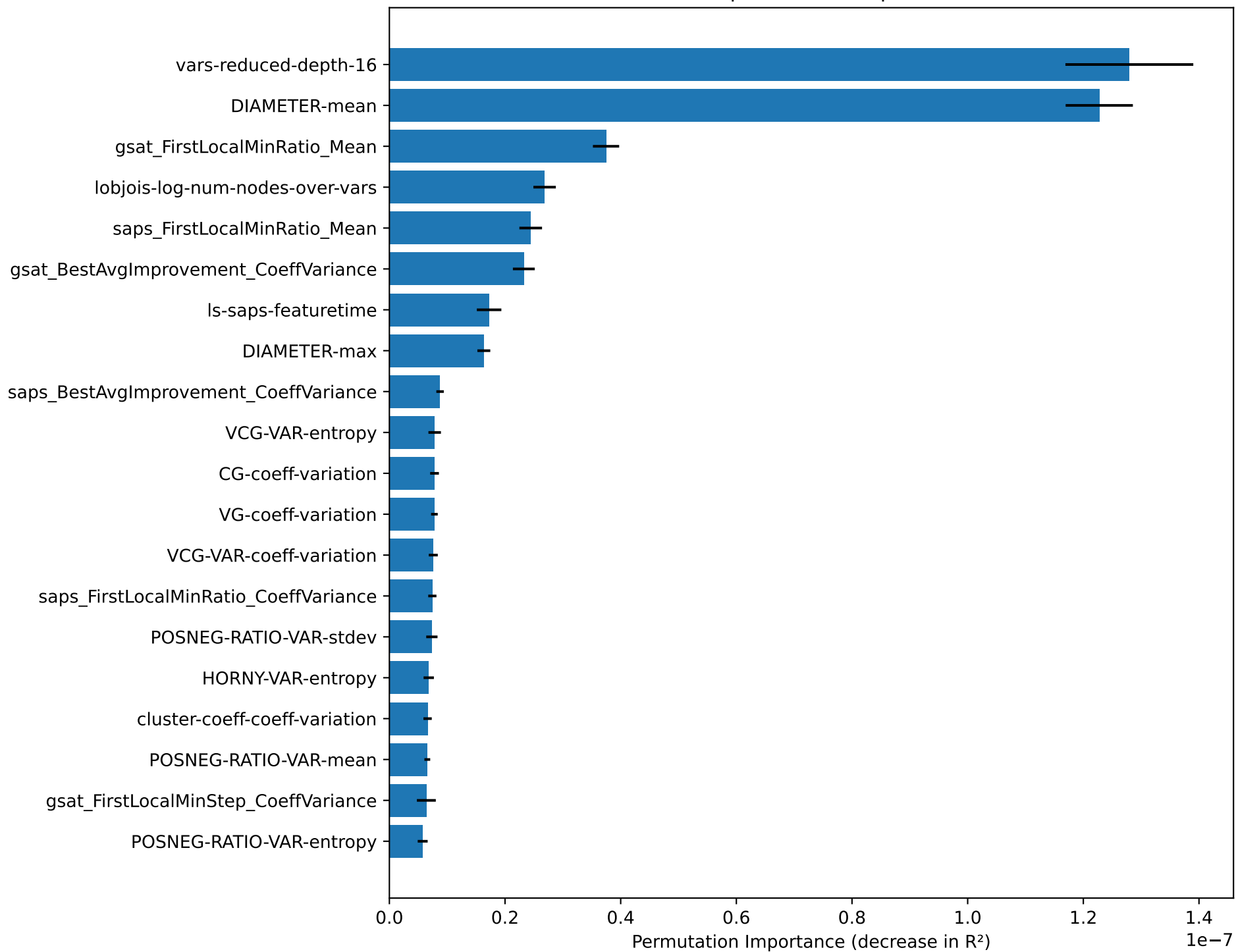
Feature Importance for Iqr Prediction
