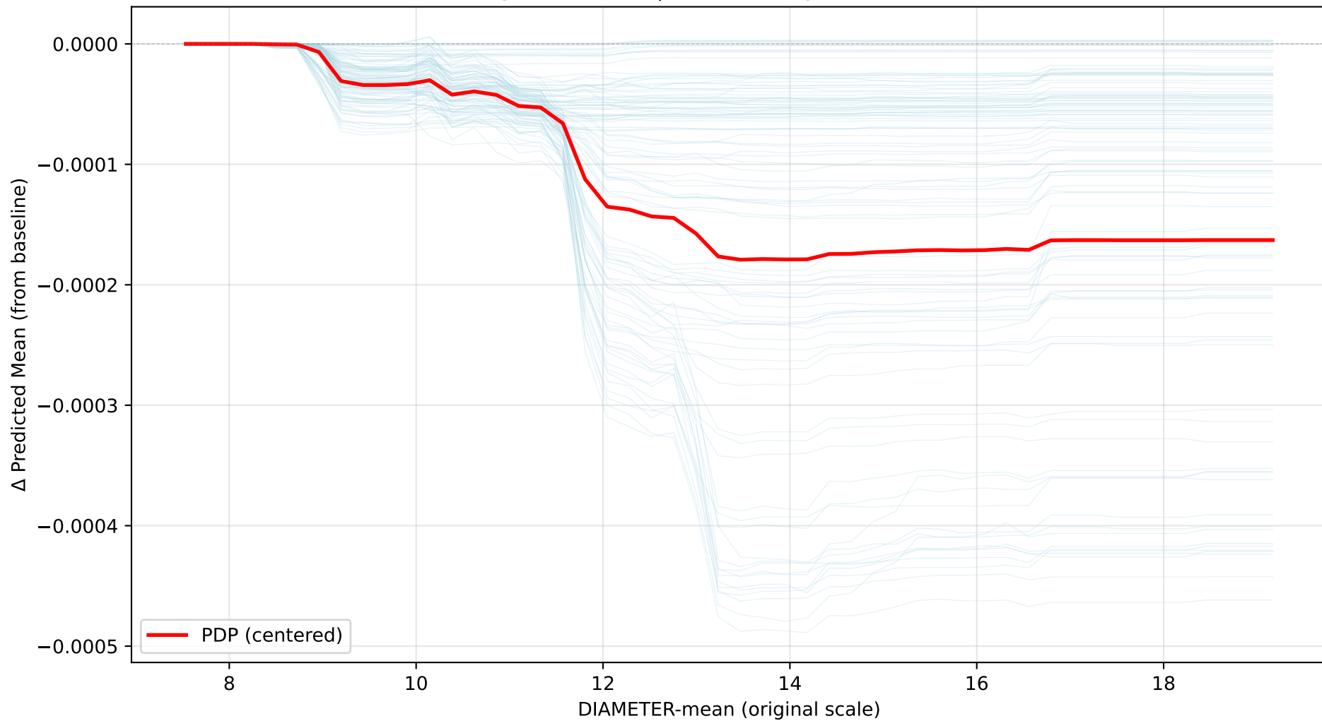
Centered ICE Curves for DIAMETER-mean (Mean) \Delta range: 0.000558 | Feature range: [7.535, 19.168]
