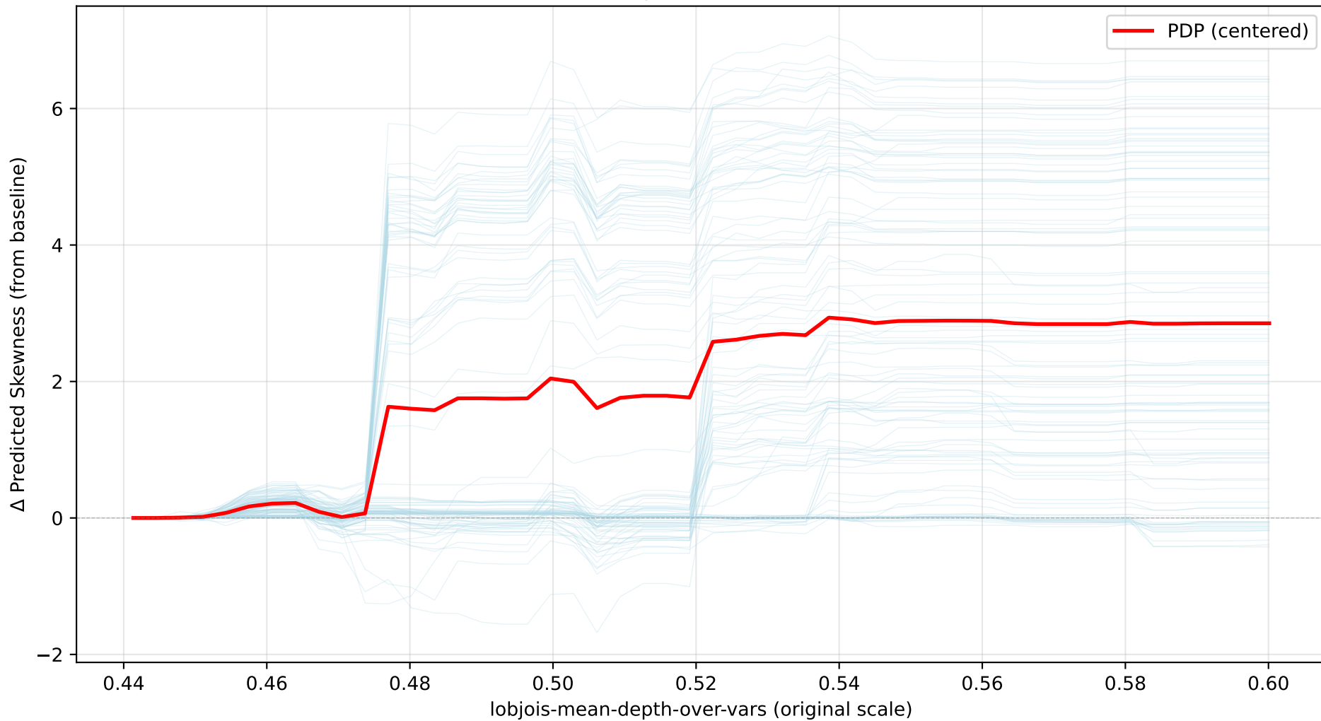
Centered ICE Curves for lobjois-mean-depth-over-vars (Skewness)
