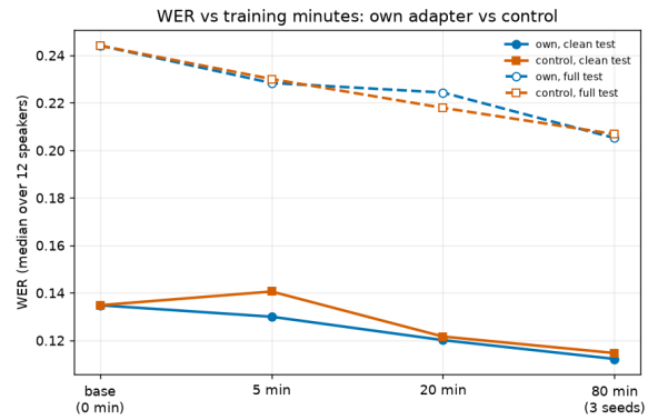
Figure 13: Median WER over the 12 speakers at 0 (arm B), 5, 20 and 80 minutes of training audio, for the own adapter (blue) and the control (orange), on the clean test (solid) and the full test (dashed). At 80 minutes, each speaker's WER is averaged over three seeds.
