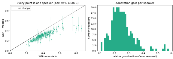
Figure 9: Left: per-speaker WER under arm A against arm B. Every point is one speaker, the bar is the 95% bootstrap interval on WER_B and the dashed line is no change. Right: distribution of the relative gain over the 261 speakers with at least 20 segments.
