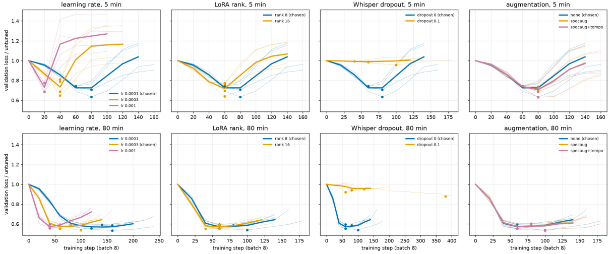
Figure 8: Validation loss relative to arm B during tuning, varying one setting at a time around the chosen recipe, at 5 minutes (top) and 80 minutes (bottom). Thin lines: the four speakers; thick: their mean; dots: the best checkpoints.
