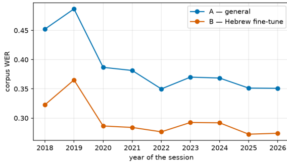
Figure 12: Corpus WER of both models by the year of the session, after the quality filter.
