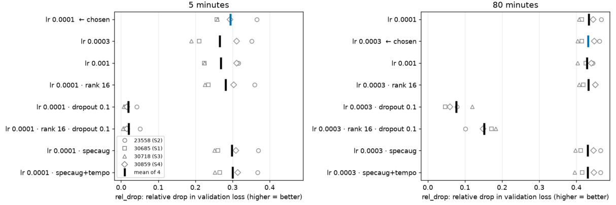
Figure 7: Every tuning run, at 5 minutes (left) and 80 minutes (right). Markers: the four tuning speakers; bar: their mean; blue: the chosen setting. The x-axis is the relative drop in validation loss from arm B to the best checkpoint.
