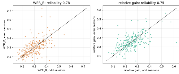
Figure 10: Each point is one speaker, measured separately on their odd and even sessions. Points near the diagonal mean the measure repeats across recordings, and titles give the split-half reliability (Spearman–Brown corrected).
