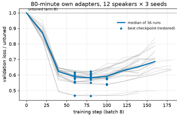
Figure 6: Validation loss relative to arm B while training the 80-minute own adapters (12 speakers \times 3 seeds). Thin lines: one run each; thick: the median; dots: the checkpoints early stopping restored.
