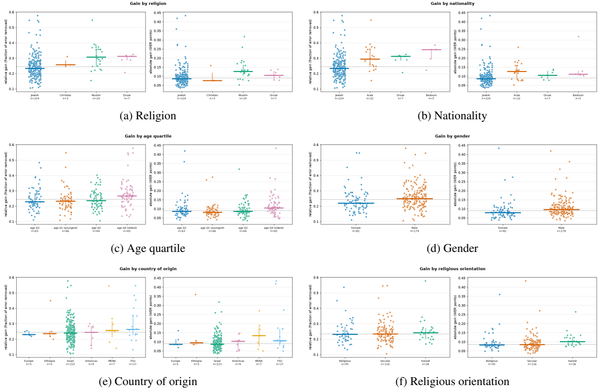
Figure 11: Gain from the Hebrew fine-tune by group, relative (left of each panel) and absolute (right). Each point is one speaker with at least 20 segments. The bar is the group median, the line the interquartile range, and the dashed line the overall median.
