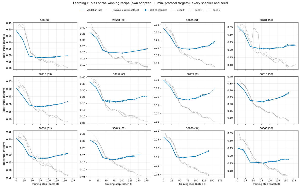
Figure 15: Learning curves of the 80-minute own adapters, one panel per speaker. Blue: validation loss every 20 steps (step 0 is arm B); grey: training loss, smoothed over 20 steps; line style: seed; dot: the checkpoint early stopping restored.
