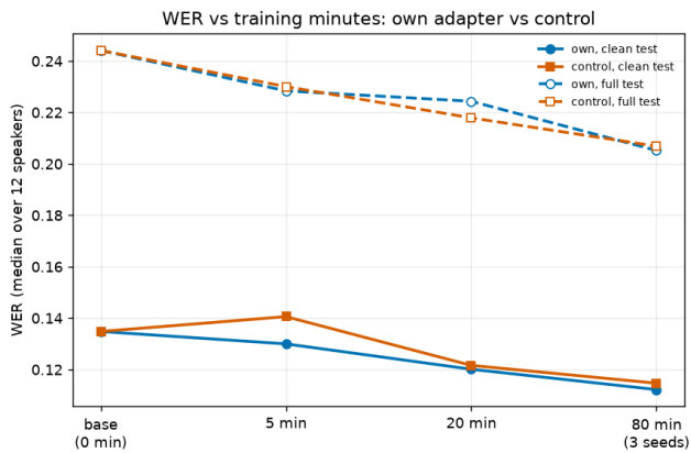
Figure 13: Median WER over the 12 speakers at 0 (arm B), 5, 20 and 80 minutes of training audio. At 80 minutes, each speaker's WER is averaged over three seeds.
