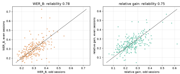
Figure 9: Each point is one speaker, measured separately on their odd and even sessions. Points near the diagonal mean the measure repeats across recordings, and titles give the split-half reliability (Spearman-Brown corrected).
