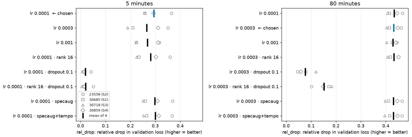
Figure 6: Every tuning run, at 5 minutes (left) and 80 minutes (right). Markers are the four tuning speakers, the bar is their mean, and blue is the chosen setting. The x-axis is the relative drop in validation loss from arm B to the best checkpoint.
