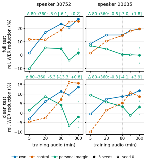
Figure 15: As Figure 5, for the two speakers trained on up to 360 minutes.
