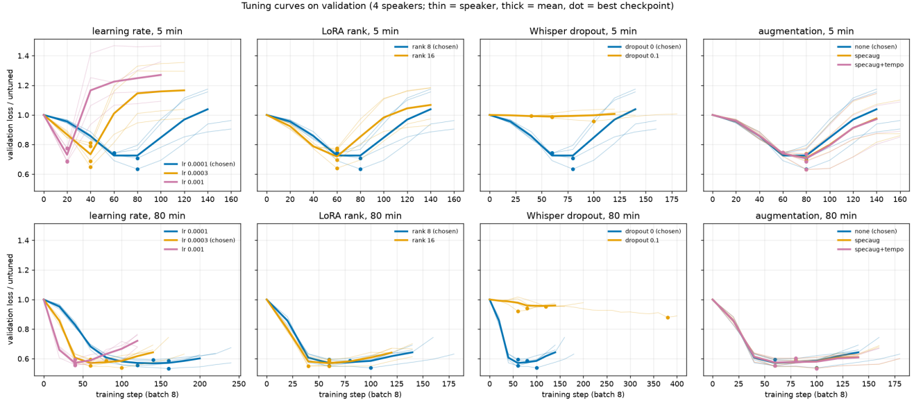
Figure 7: Validation loss relative to arm B during tuning, varying one setting at a time around the chosen setting, at 5 minutes (top) and 80 minutes (bottom). Thin lines are the four speakers, the thick line is their mean, and dots are the best checkpoints.
