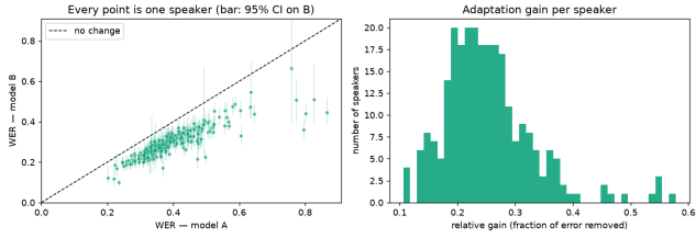
Figure 8: Left: per-speaker WER under arm A against arm B. Every point is one speaker, the bar is the 95% bootstrap interval on WER_B and the dashed line is no change. Right: distribution of the relative gain over the 261 speakers with at least 20 segments.
