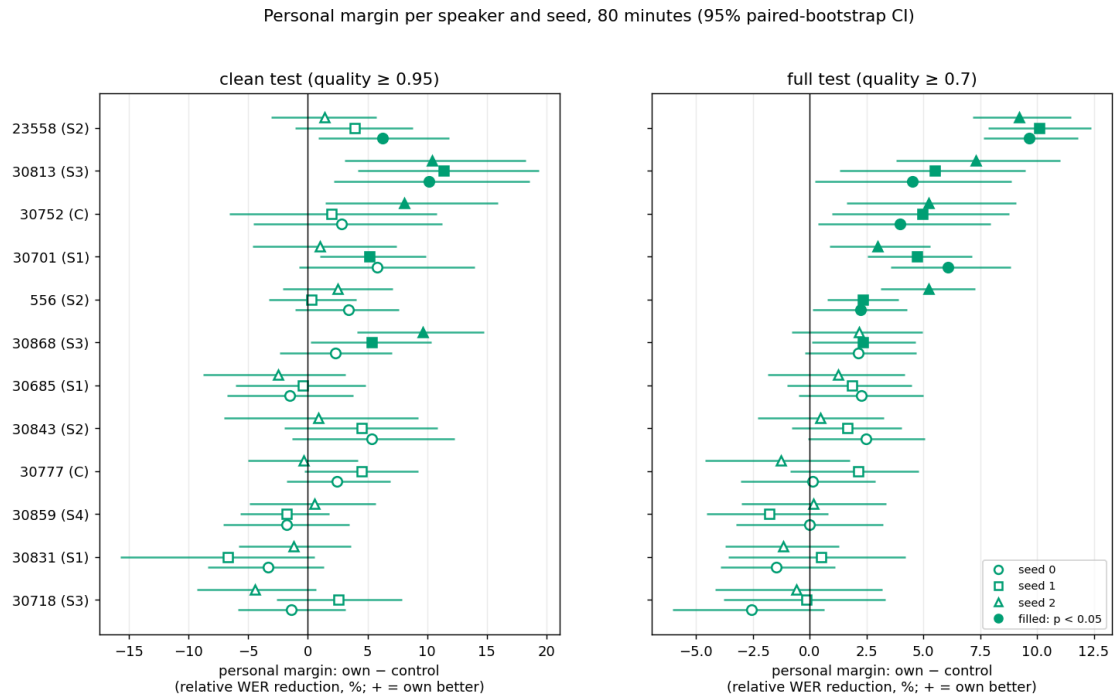
Figure 12: Personal margin per speaker and seed at 80 minutes, with 95% paired-bootstrap intervals. Filled markers are significant ( p < 0.05 ). Profiles: S1, helped least by the fine-tune, S2, hard under both models, S3, typical, S4, low WER, and C, served well by the fine-tune.
