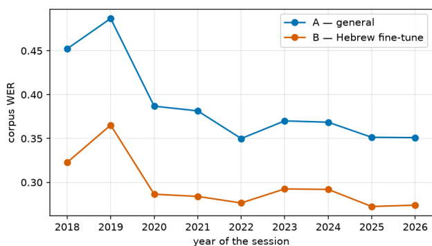
Figure 11: Overall WER of both models by the year of the session, after the quality filter.
