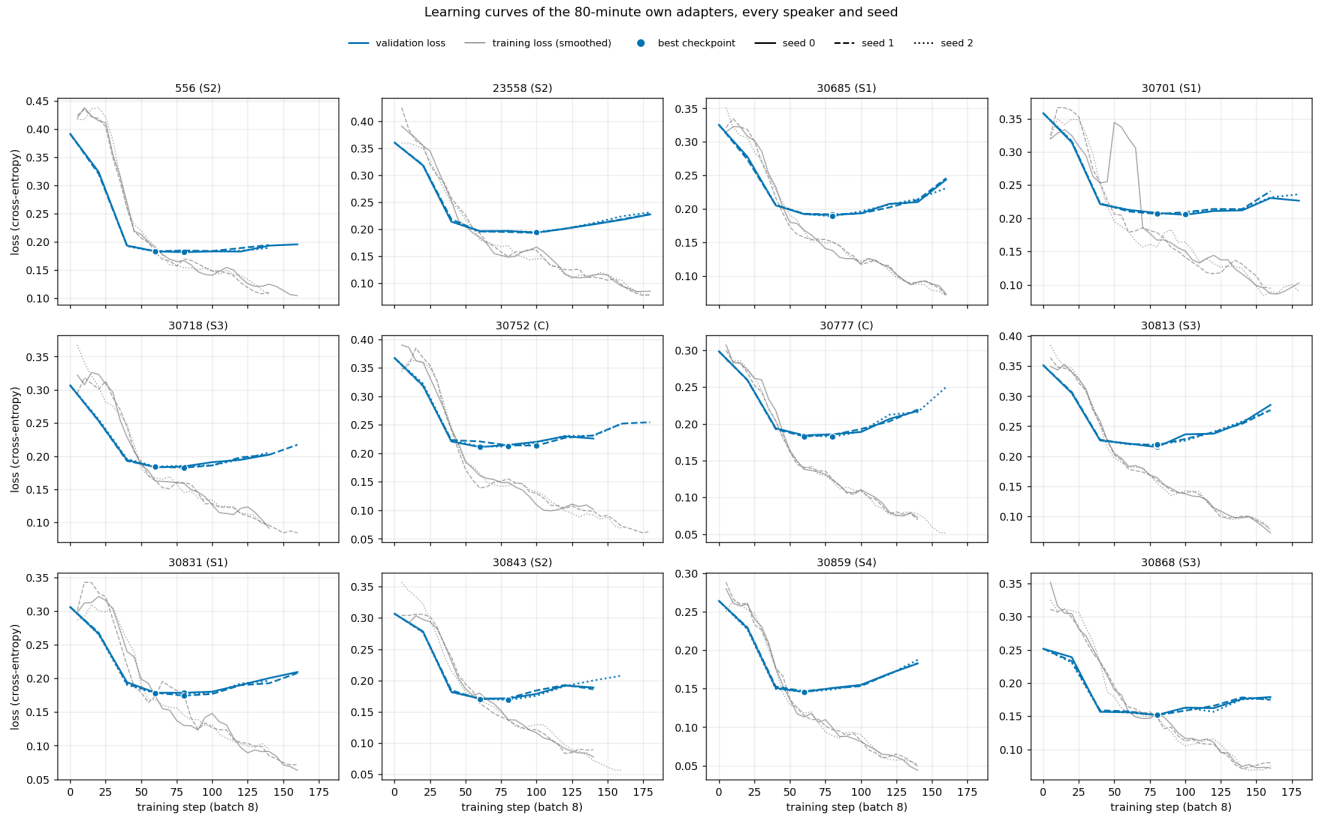
Figure 14: Training and validation loss of the 80-minute own adapters, one panel per speaker. Step 0 is arm B.
