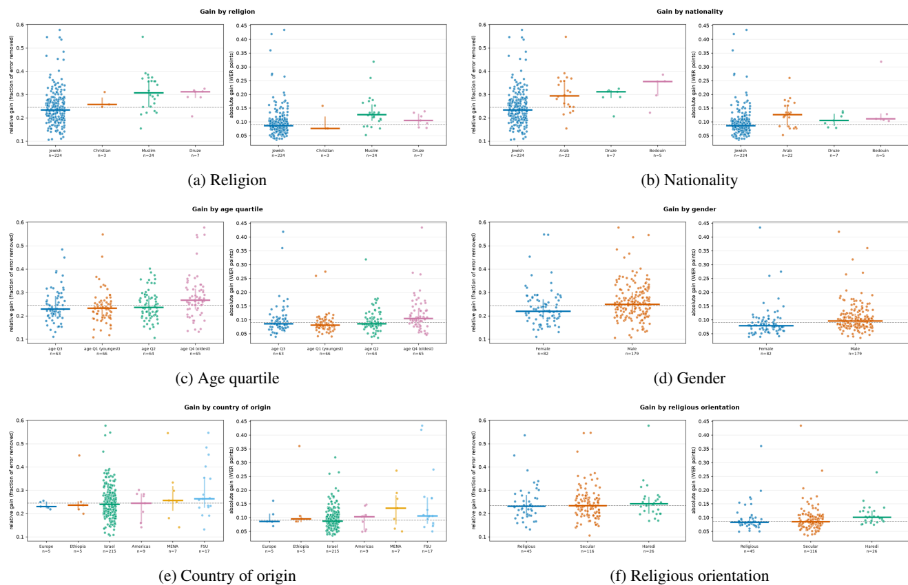
Figure 10: Gain from the Hebrew fine-tune by group, relative (left of each panel) and absolute (right). Each point is one speaker with at least 20 segments. The bar is the group median, the line the interquartile range, and the dashed line the overall median.
