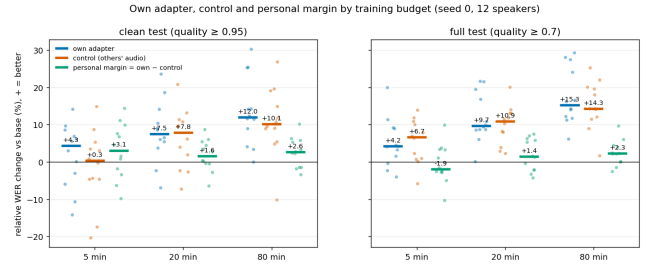
Figure 3: Relative WER change over arm B at 5, 20 and 80 minutes of training audio (seed 0, 12 speakers). Each dot is one speaker, and bars and numbers are medians. The median personal margin is the median of per-speaker differences.
