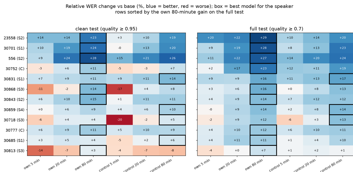
Figure 4: Relative WER change over arm B (%) for each speaker under each adapter, with the speaker’s lowest WER boxed. The 80-minute columns average three seeds.
