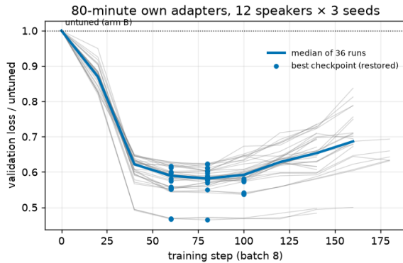
Figure 7: Validation loss relative to arm B while training the 80-minute own adapters (12 speakers \times 3 seeds). Thin lines: one run each; thick: the median; dots: the checkpoints early stopping restored.
