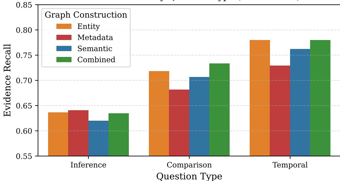
Evidence Recall by Question Type ( k = 17 PCST)
