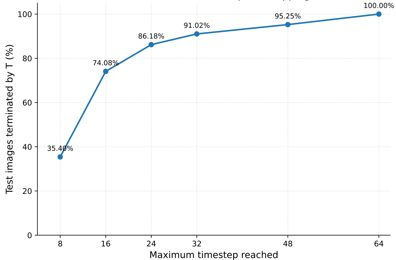
Cumulative Distribution of Adaptive Stopping Times
