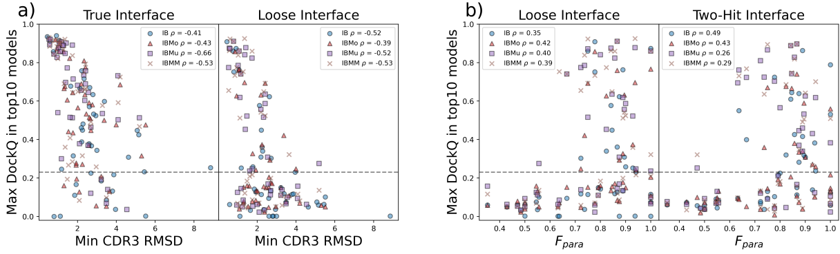
Figure 4: Nanobody structural quality and paratope definition are related to docking success. a) Scatter plot between the minimum CDR3 RMSD in the input models and the maximum DockQ achieved among the top10 models for each ensemble. Analysed models come from True Interface scenario and bound antigen. Pearson correlation coefficients for each ensemble are reported on the top right. The horizontal dashed line in each plot indicates a DockQ of 0.23, which is the cutoff used to define acceptable or better models. b) Scatter plots showing the relationship between the fraction of paratope present in the restraints ( F_{para} ) and the maximum DockQ among the top 10 models for each ensemble. Data are shown for both Loose and Two-Hit Interface scenarios. Pearson correlation coefficients are plotted on the top left.
