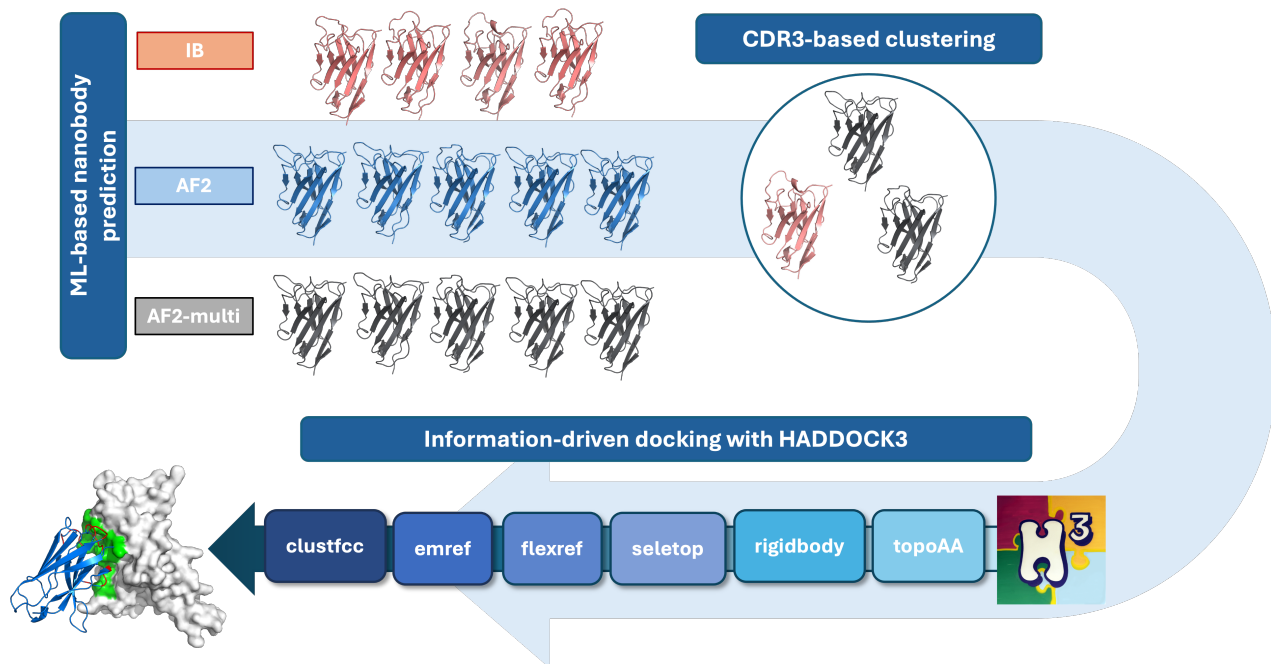
Figure 1: Graphical representation of the nanobody-antigen complex prediction pipeline. First, nanobody conformations are generated using AlphaFold (AF2), AlphaFold2-Multimer (AF2-multi) and ImmuneBuilder (IB). Those are then clustered based on the similarity of the CDR3 loop and passed to HADDOCK for ensemble-based information-driven docking using CDR loop residues and some knowledge of the epitope to define ambiguous interaction restraints to drive the modelling process.
