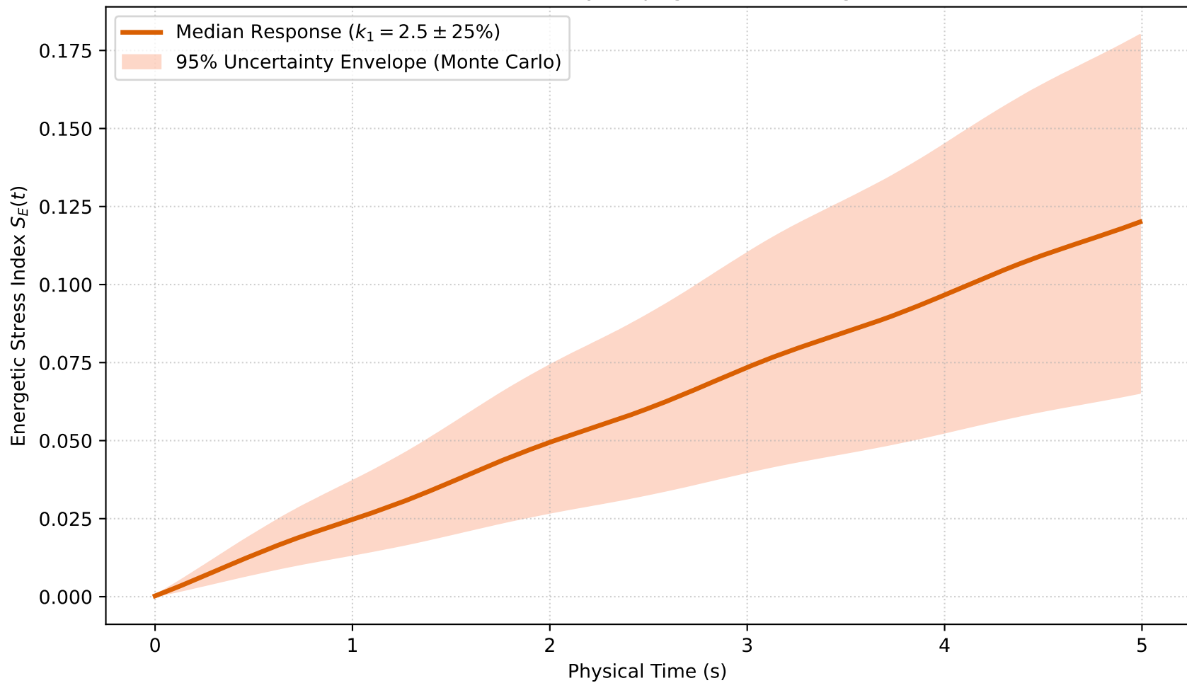
Monte Carlo Uncertainty Propagation for Energetic Stress
