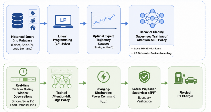
Fig. 3. End-to-end framework: offline LP distillation, composite imitation training, and online real-time edge execution with deterministic SPP projection.
