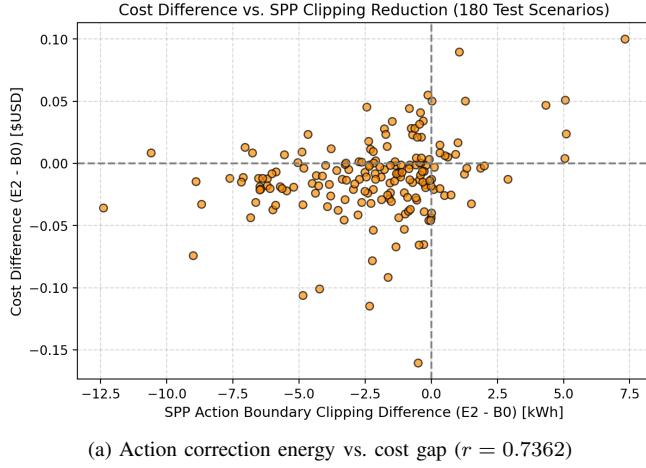
Fig. 2. Empirical forensic analysis across 180 frozen test scenarios: (a) scatter relationship between Action Boundary Correction Energy and economic gap ( r = 0.7362 , p = 5.33 \times 10^{-32} ); and (b) closed-loop mechanism of SPP-induced State-of-Charge trajectory drift.
