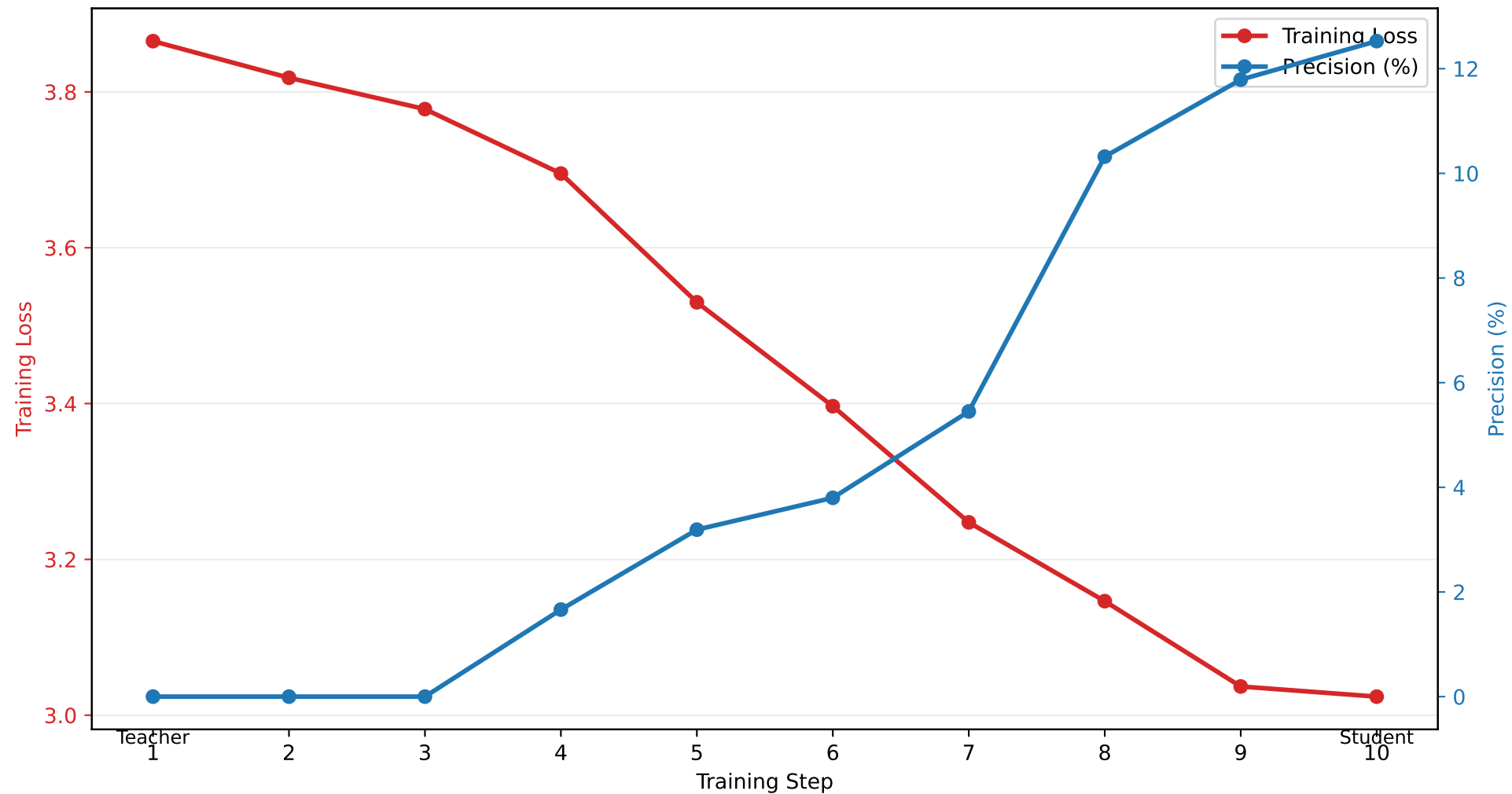
Loss and Precision vs. Training Step
