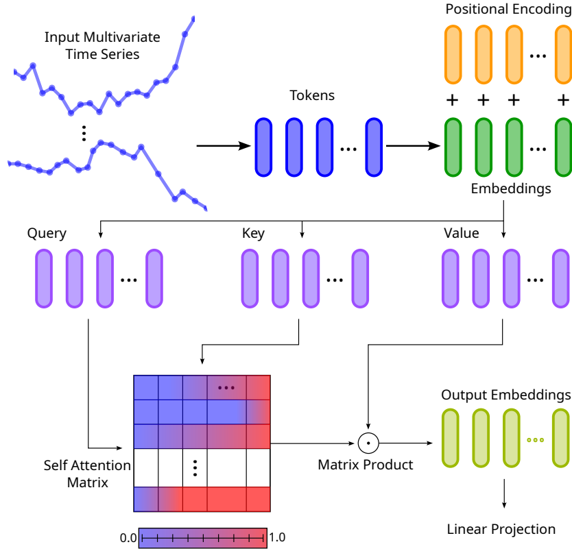
Fig. 8. Temporal Self-Attention applied on a multivariate time series.
