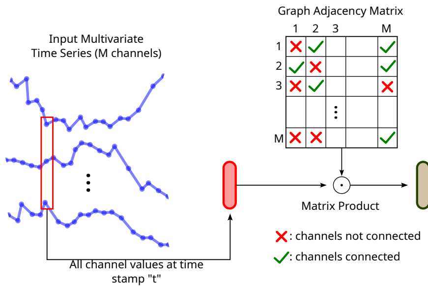
Fig. 7. Graph operation applied on a multivariate time series.
