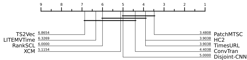
Fig. 12. A comparison of ranks of nine classifiers on 26 equal length datasets.
