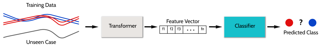
Fig. 1. Example of a pipeline-based time series classifier.
