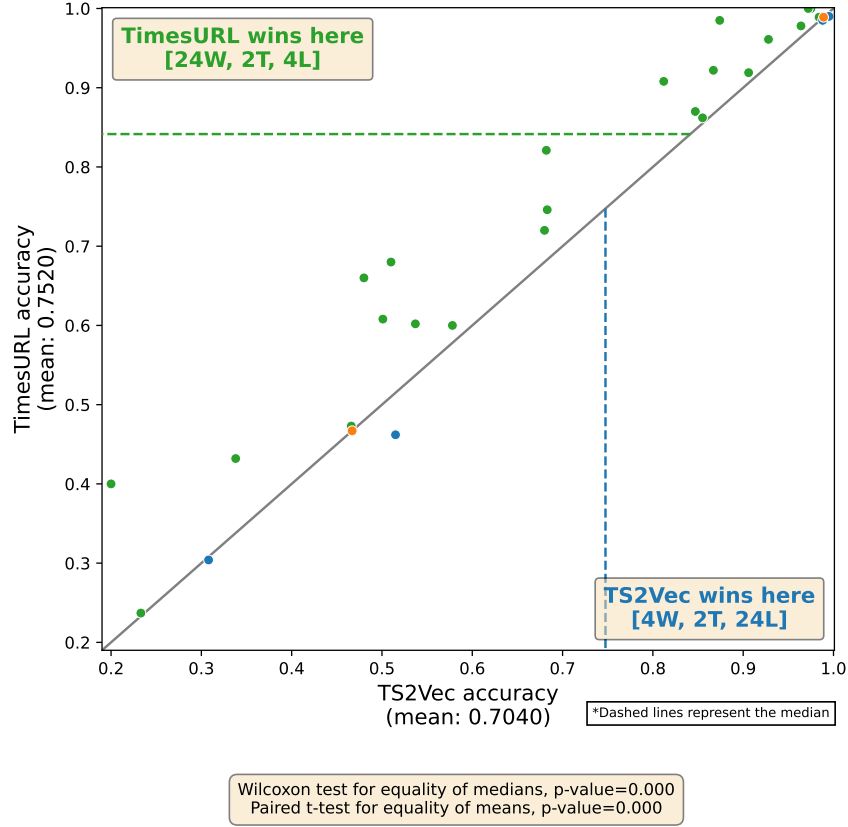
Fig. 11. A scatter plot of test set accuracies of TimesURL vs TS2Vec.
