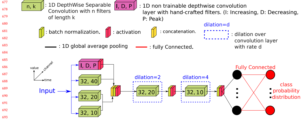
Fig. 5. The LITEMV architecture (taken from [56] with permission).
