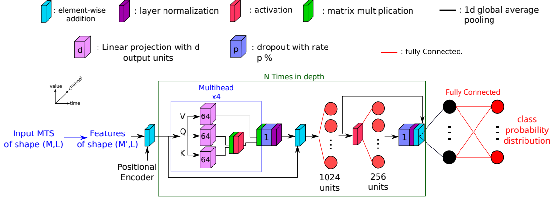
Fig. 9. The Vanilla Transformer (VanTran) architecture for Rehabilitation MTSC, taken from [56] with permission.
