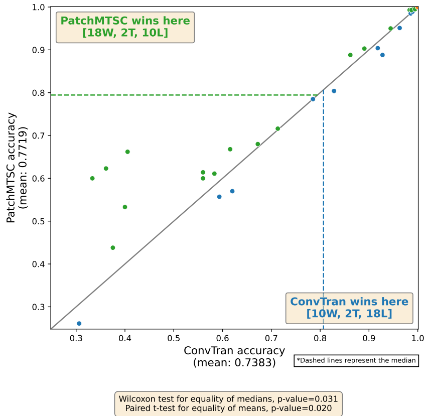
Fig. 10. A scatter plot of test set accuracies of PatchMTSC vs ConvTran.
