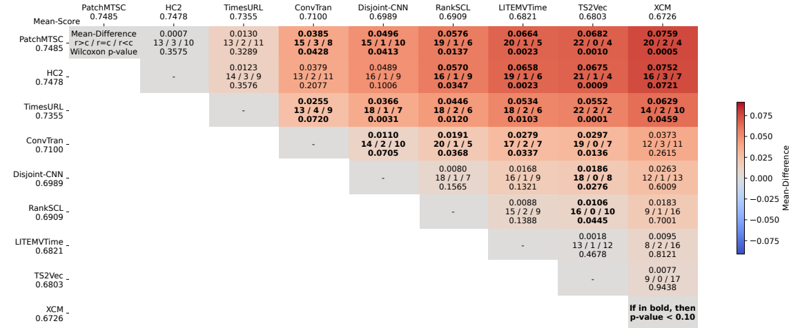
Fig. 13. A Multi-Comparison Matrix (MCM) [55] of relative performances of nine classifiers on 26 equal length datasets.
