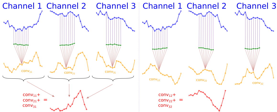
Fig. 4. One dimensional convolution applied on a multivariate time series (taken from [54] with permission).
