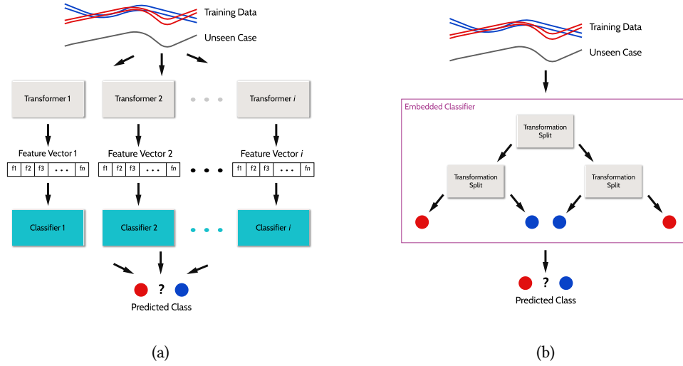
Fig. 2. Examples of machine-learning time series classifiers: (a) an ensemble-based classifier, and (b) an embedded or integrated classifier.
