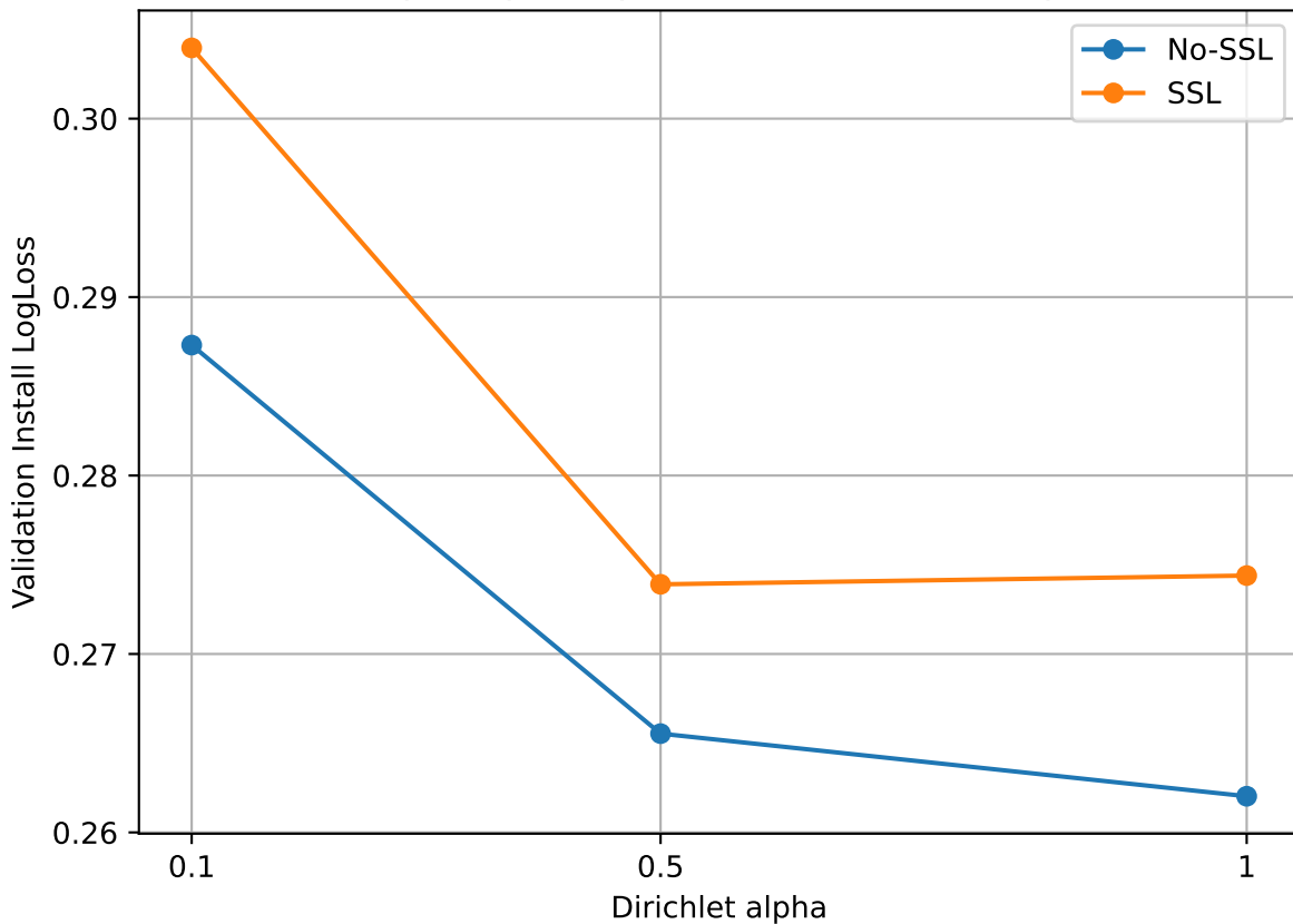
Final validation Install LogLoss vs Dirichlet alpha (best checkpoint per experiment, validation only, seed 42)
