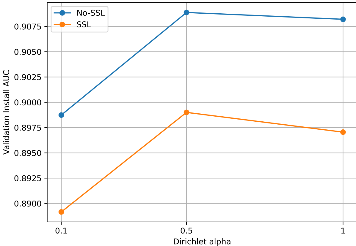
Final validation Install AUC vs Dirichlet alpha (best checkpoint per experiment, validation only, seed 42)
