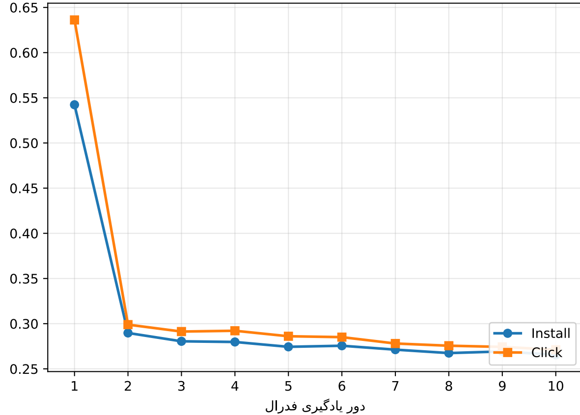
logloss
