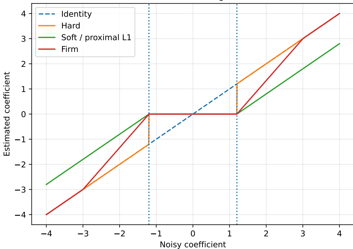
Coefficient shrinkage rules
