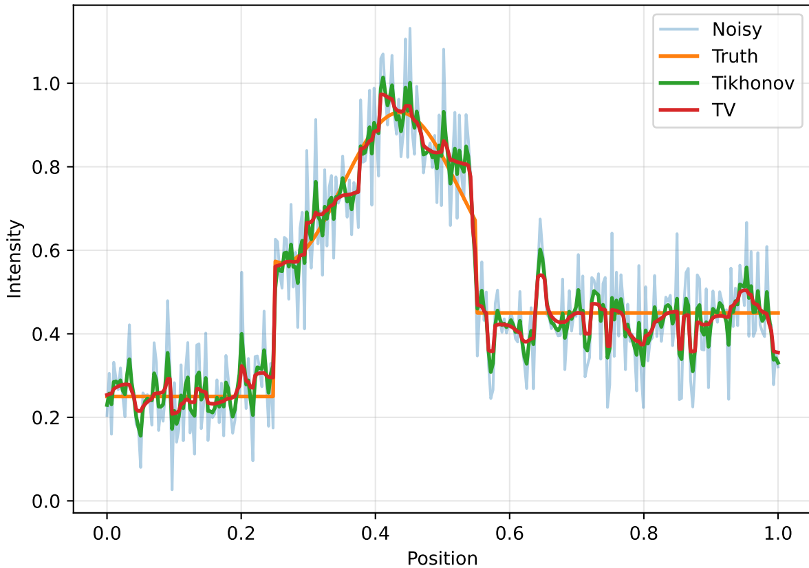
Quadratic smoothness versus total variation
