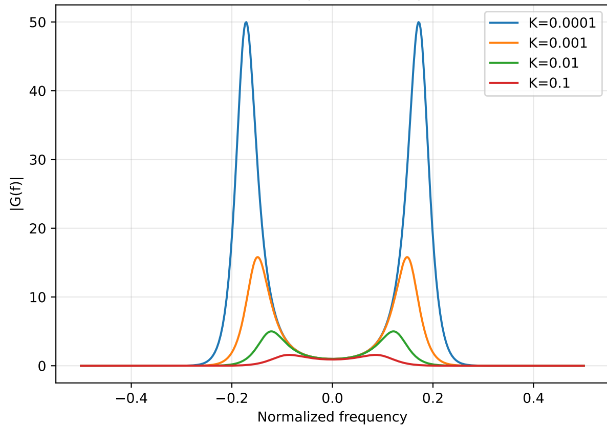
Wiener inverse response and regularization
