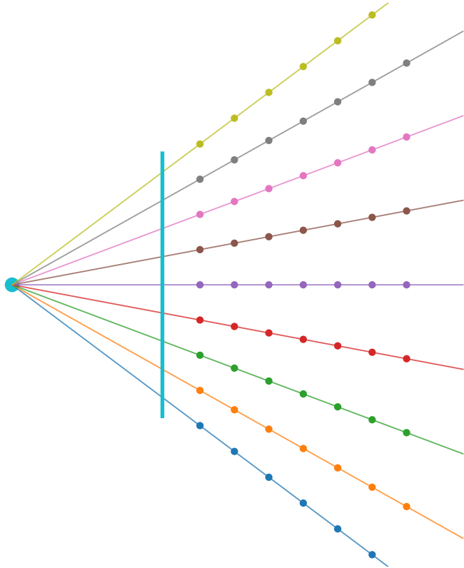
camera rays and differentiable volume samples
