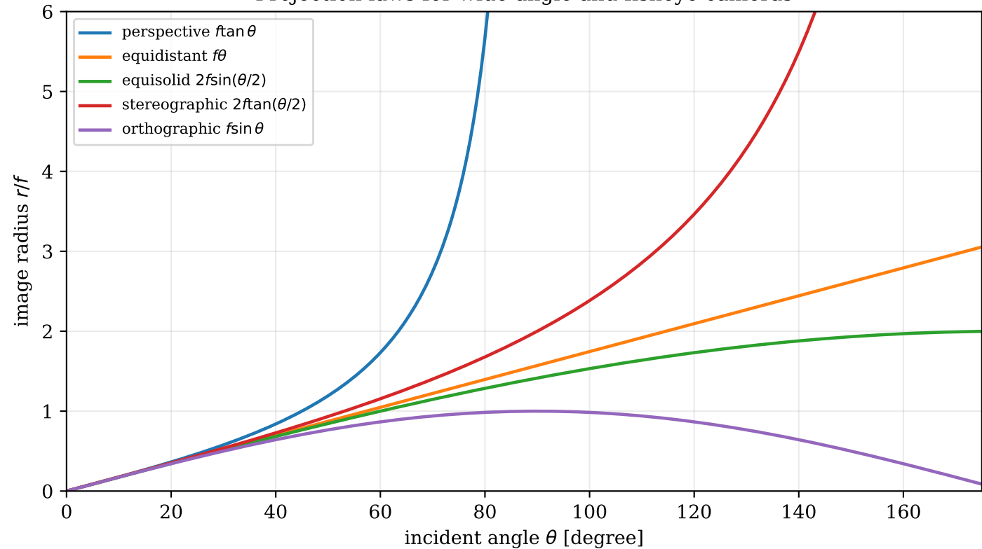
Projection laws for wide-angle and fisheye cameras
