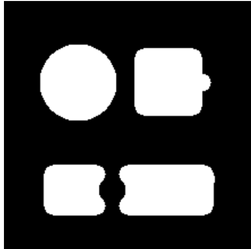
opening X \circ B
