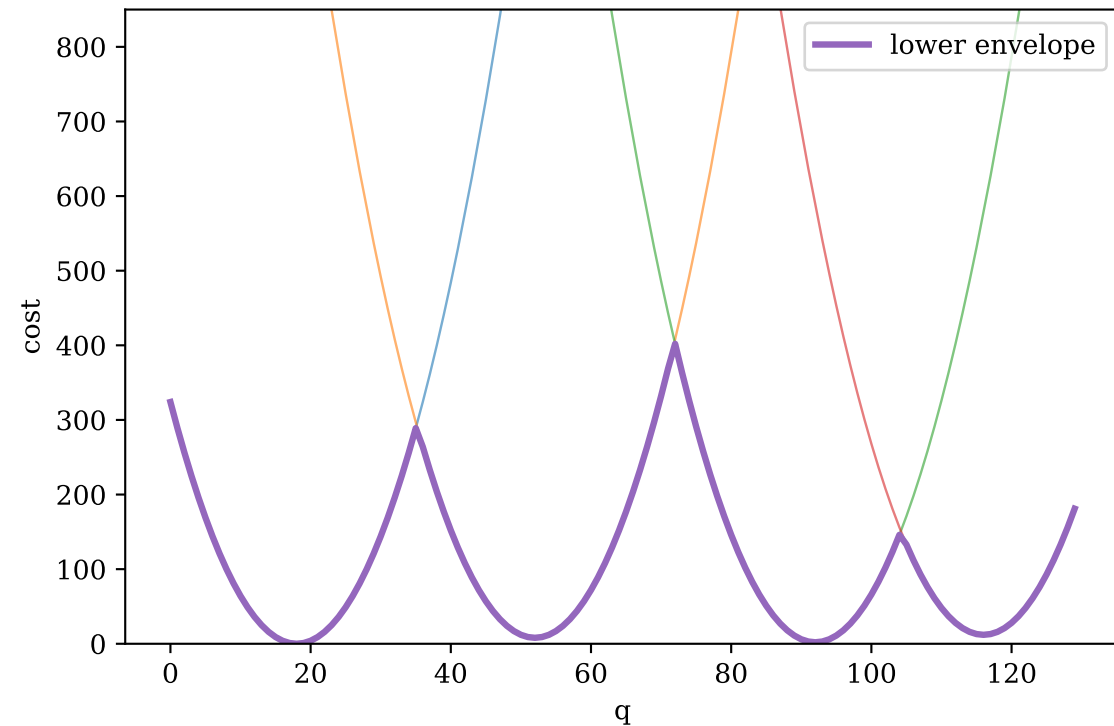
1-D exact squared distance transform
