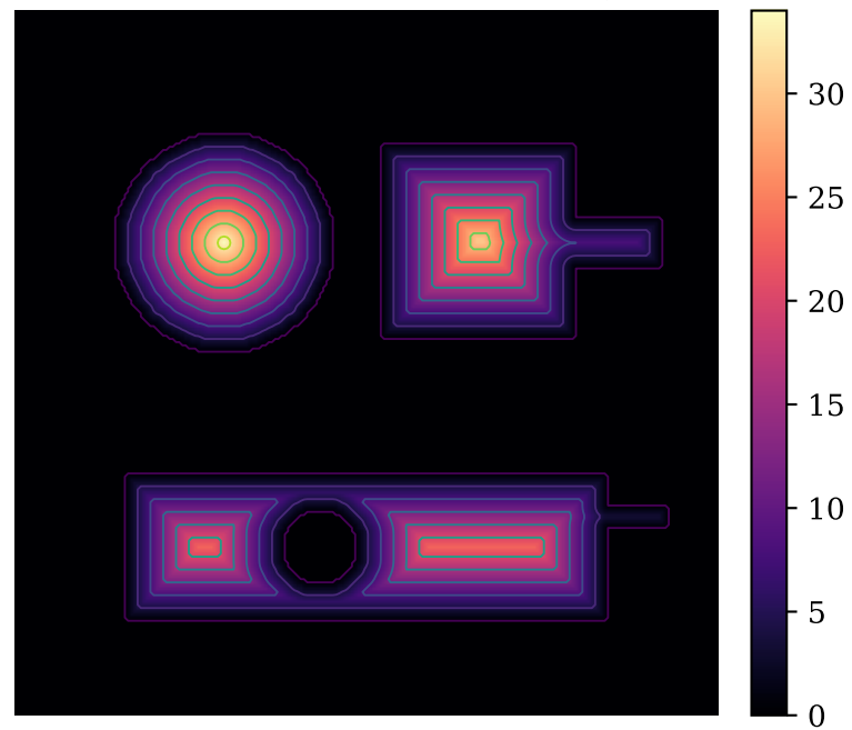
Euclidean distance inside a binary set
