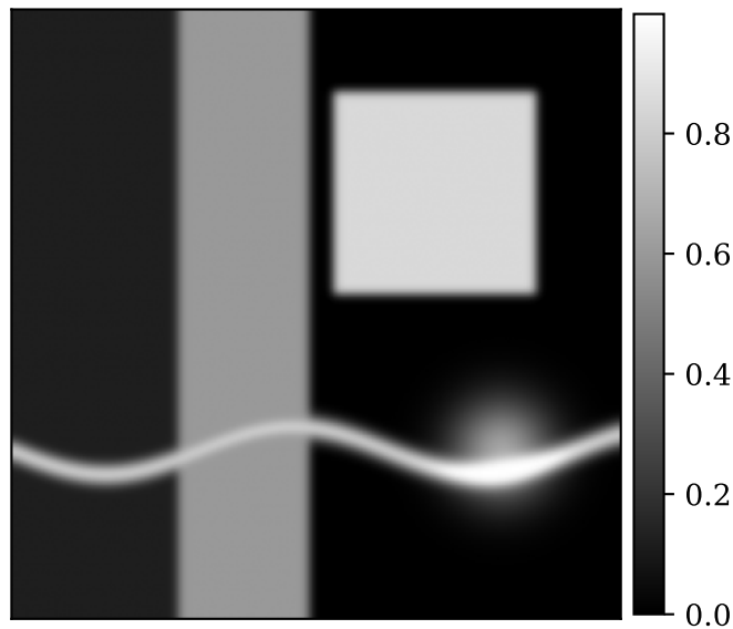
Gaussian scale-space
