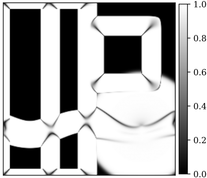
tensor coherence
