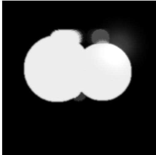
ordinary opening
