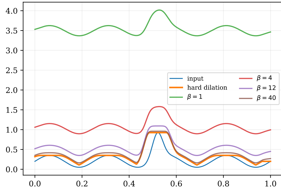
LogSumExp relaxation of dilation
