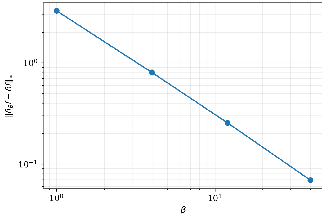
convergence to max-plus morphology
